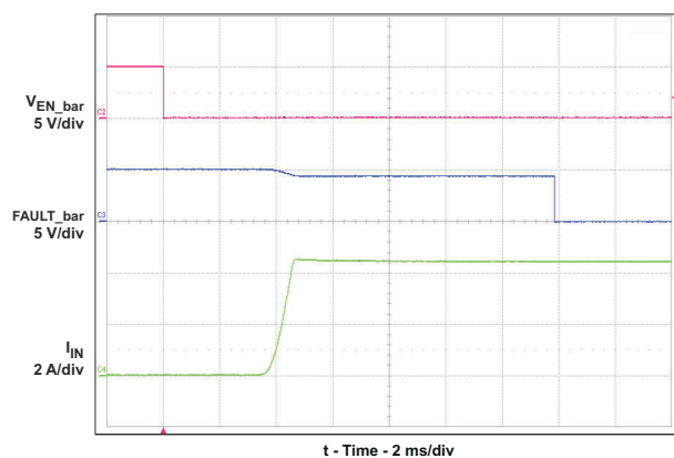
10-5. Device Enabled Into Short Circuit
