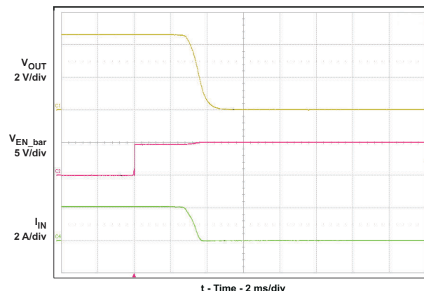
10-4. Turnoff Delay and Fall Time
