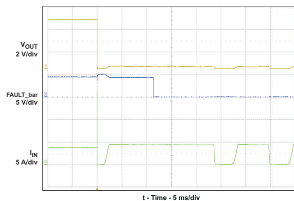
10-6. Full-Load to Short-Circuit Transient Response
