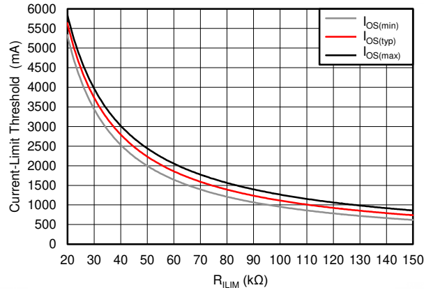
FIG 10-2. Current-Limit Threshold versus R_{(ILIM)}
