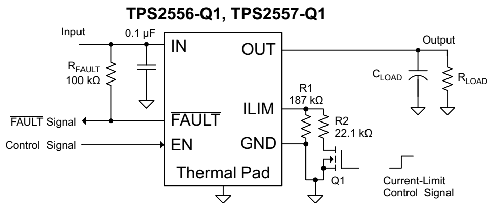
FIG 9-3. Two-Level Current-Limit Circuit
