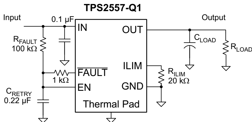
FIG 9-1. Auto-Retry Functionality
