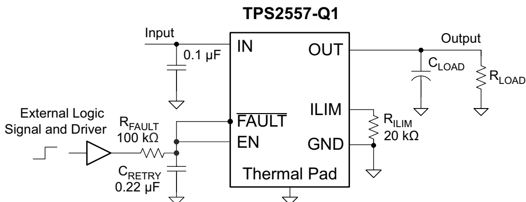
FIG 9-2. Auto-Retry Functionality With External EN Signal
