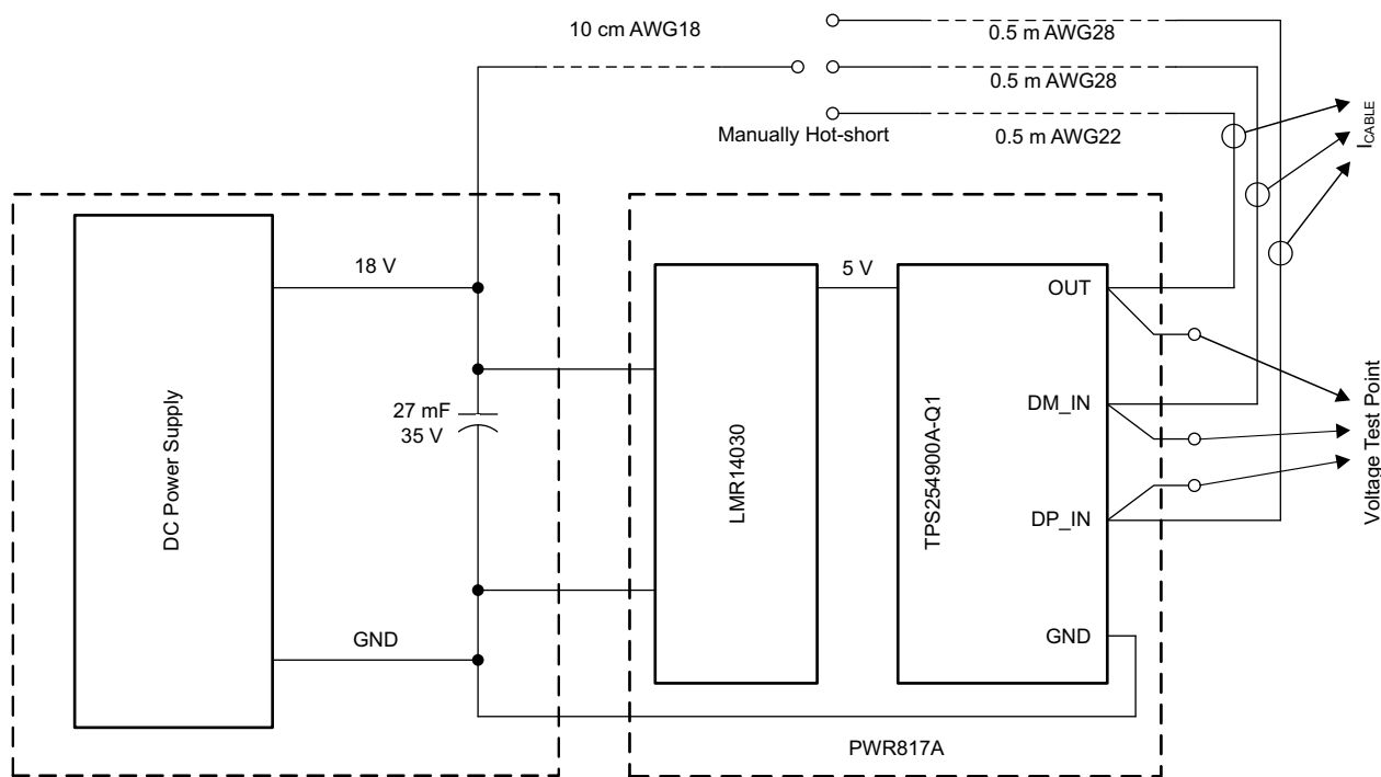
Figure 7-1. Short-to-Battery System Test Setup
