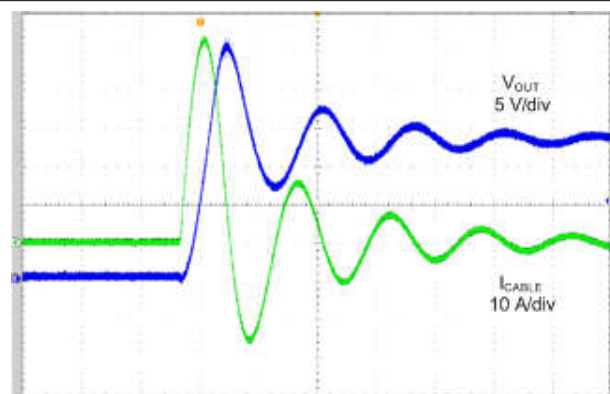
图 9-3. Disabled, 35-V, 1210, X7R C_{OUT} Capacitor Without SMAJ18
