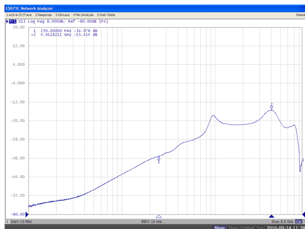
Figure 6-35. On-State Cross-Channel Isolation vs Frequency
