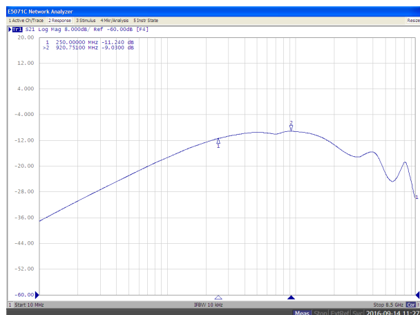
Figure 6-34. Off-State Data-Switch Isolation vs Frequency
