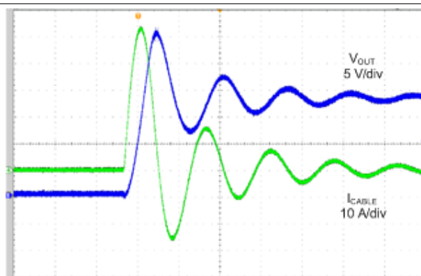
V_{BAT} = 18\text{ V} t = 10\text{ }\mu\text{s/div} Figure 45. Disabled, 35-V, 1210, X7R C_{OUT} Capacitor Without SMAJ18
