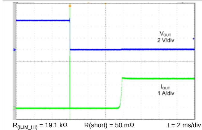
Figure 24. Hot Short
