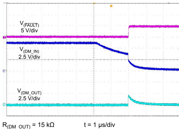
图 6-31. DM_IN Short-to-V BUS Recovery
