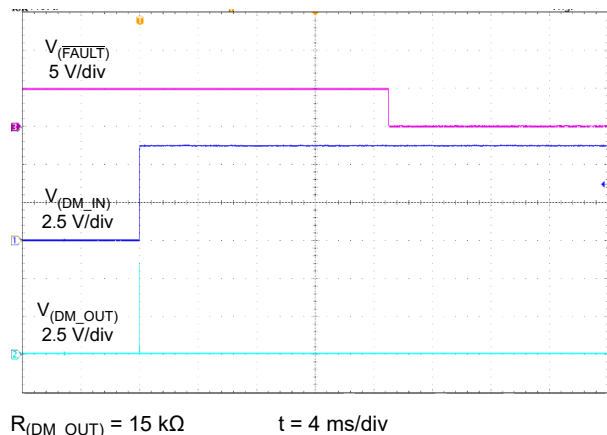
图 6-30. DM_IN Short to V BUS
