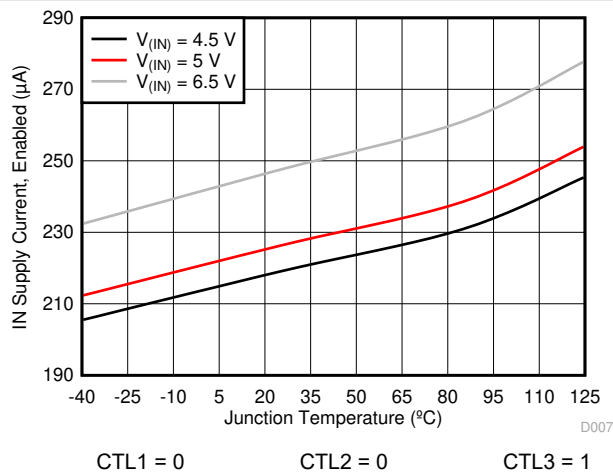
Figure 6-7. Enabled IN Supply Current – DCP_Auto (001) vs Temperature
