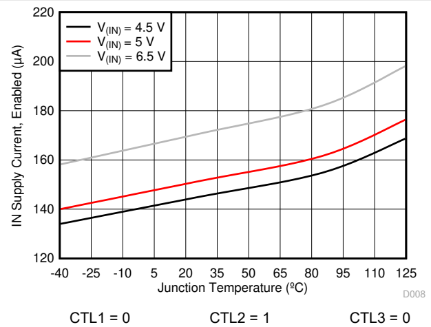
Figure 6-8. Enabled IN Supply Current – SDP (010) vs Temperature
