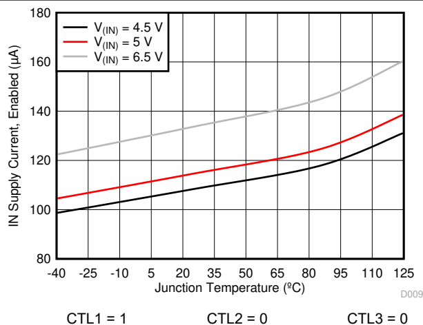
Figure 6-9. Enabled IN Supply Current – Client Mode (100) vs Temperature
