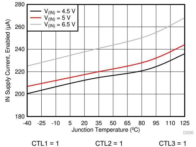
Figure 6-6. Enabled IN Supply Current – CDP (111) vs Temperature
