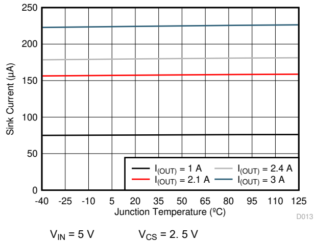
6-13. I_{CS} vs Temperature
