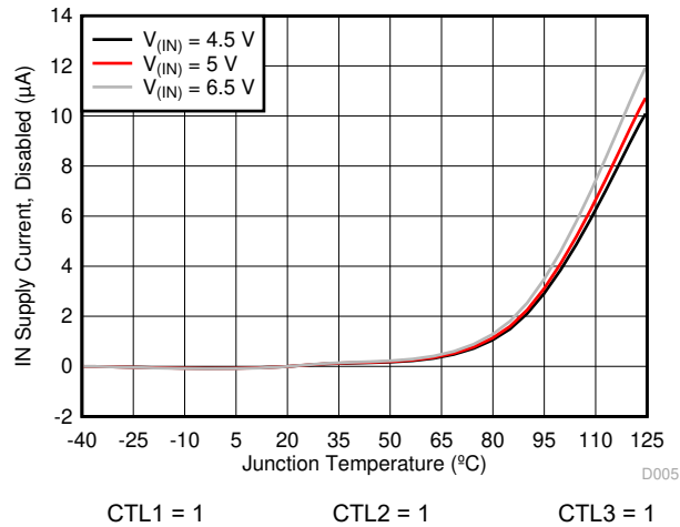
Figure 6-5. Disabled IN Supply Current vs Temperature
