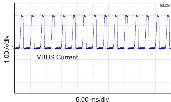
Figure 43. High-Current Limit
