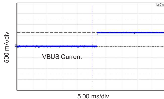
Figure 44. Low-Current Limit
