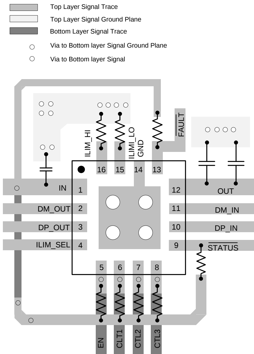
Figure 46. Layout Recommendation
