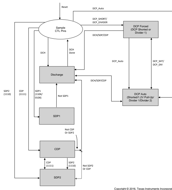
Figure 38. TPS2546-Q1 Charging States
