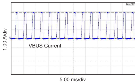
Figure 44. High-Current Limit
