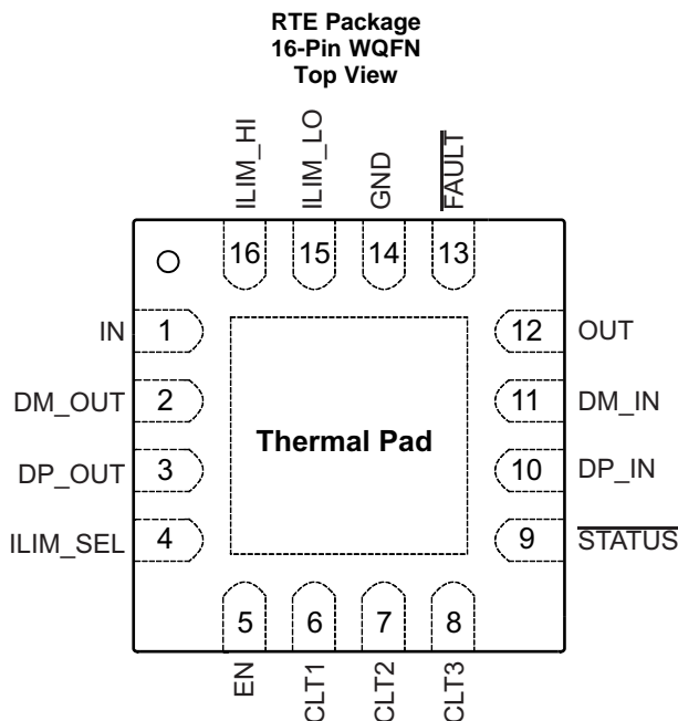
Pin Functions
