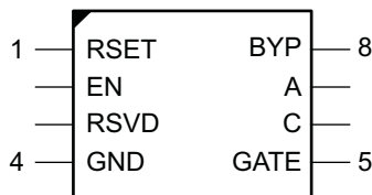
PW and D PACKAGE (TOP VIEW)
