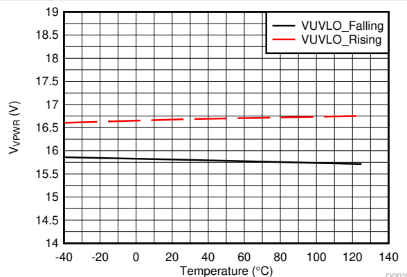
FIG 7-2. VPWR UVLO Thresholds vs Temperature
