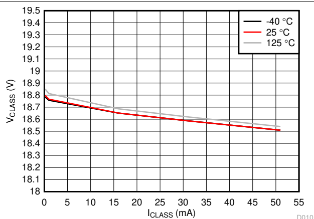
Figure 7-10. Classification Voltage vs I_{CLASS} and Temperature
