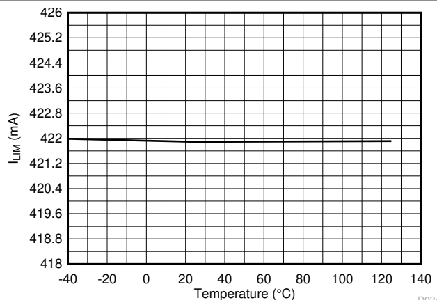
FIG 7-22. 1x Mode (2xFBn = 0) Current Limit vs Temperature
