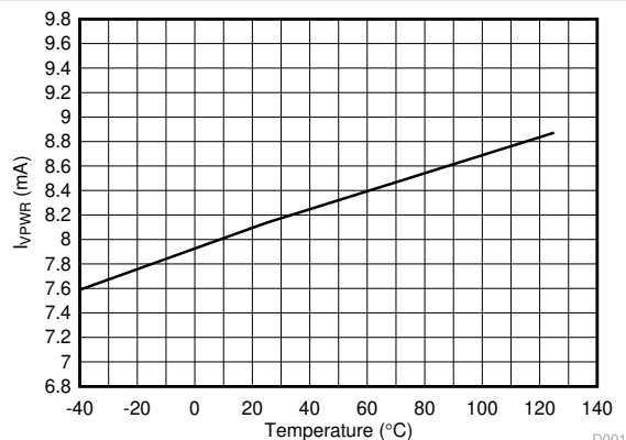
FIG 7-1. VPWR Current Consumption vs Temperature
