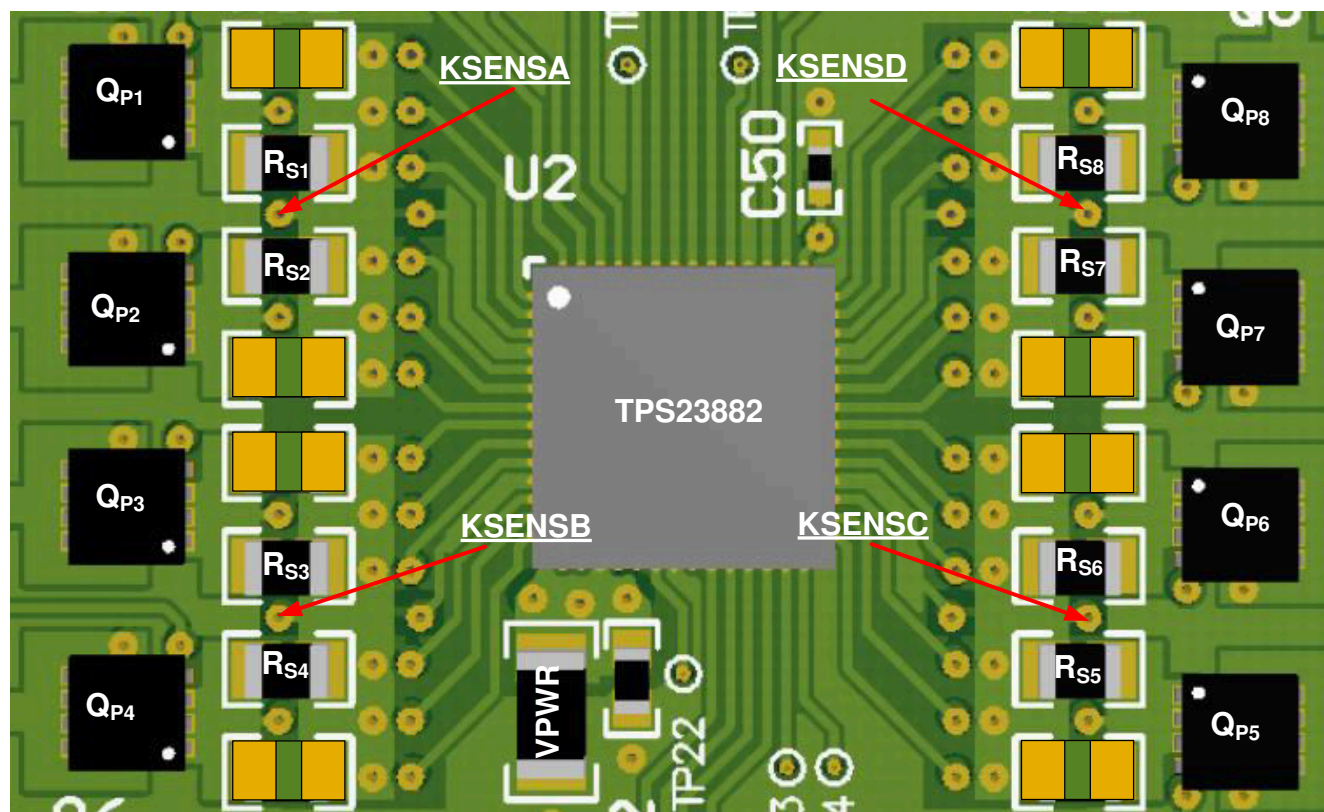
12-3. Eight Port Layout Example (Top Side)
