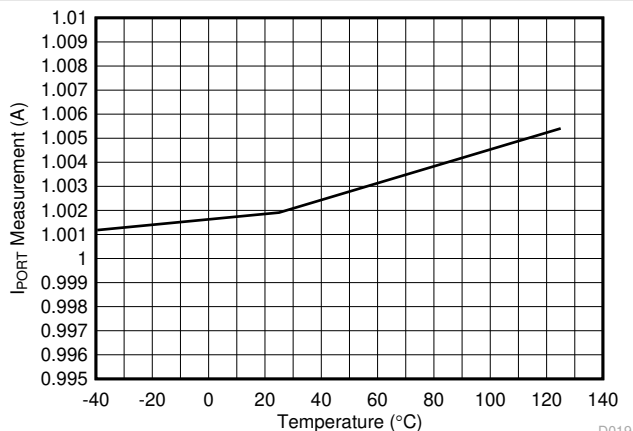
FIG 7-19. Port Current ADC Measurement (1 A) vs Temperature
