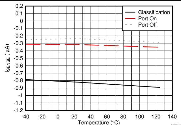
FIG 7-6. SENSE Pin Bias Current vs Temperature
