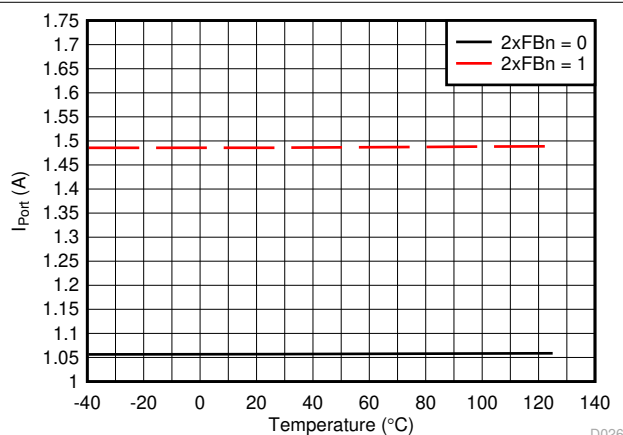
FIG 7-24. I_{\text{SHORT}} Threshold vs Temperature
