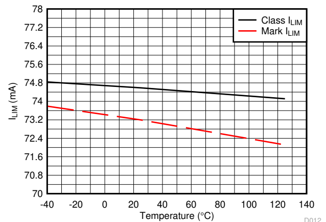
Figure 7-12. Classification and Mark Current Limit vs Temperature
