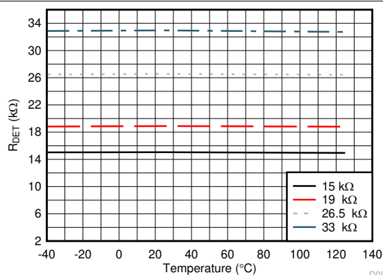
Figure 7-8. Discovery Resistance Measurement vs Temperature
