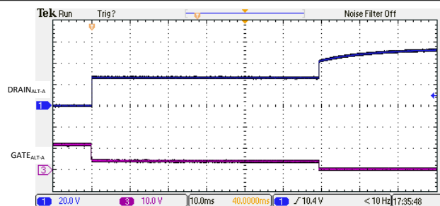
10-3. I_{LIM} Foldback and Turn-Off
