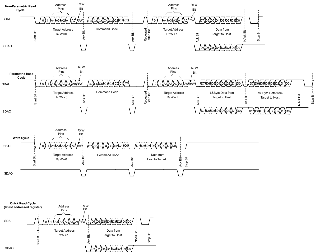
Figure 9-4. I 2 C interface Read and Write Protocol – Configuration A
