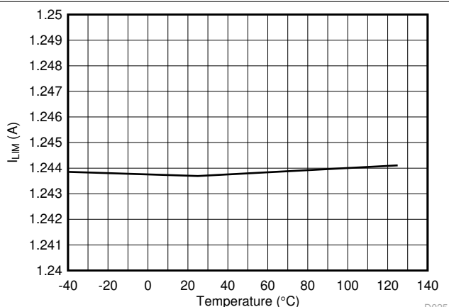
FIG 7-23. 2x Mode ( 2x\text{FBn} = 1 ) Current Limit vs Temperature
