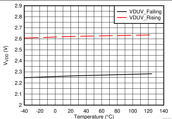
FIG 7-5. VDUV Thresholds vs Temperature
