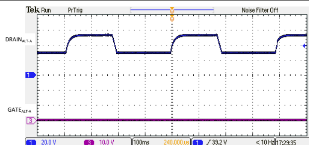
10-5. Open Circuit Detection Signature
