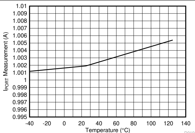
FIG 7-19. Port Current ADC Measurement (1 A) vs Temperature
