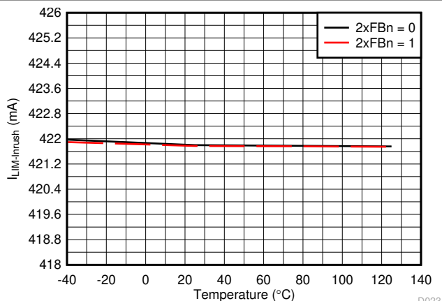
FIG 7-21. Inrush Current Limit vs Temperature
