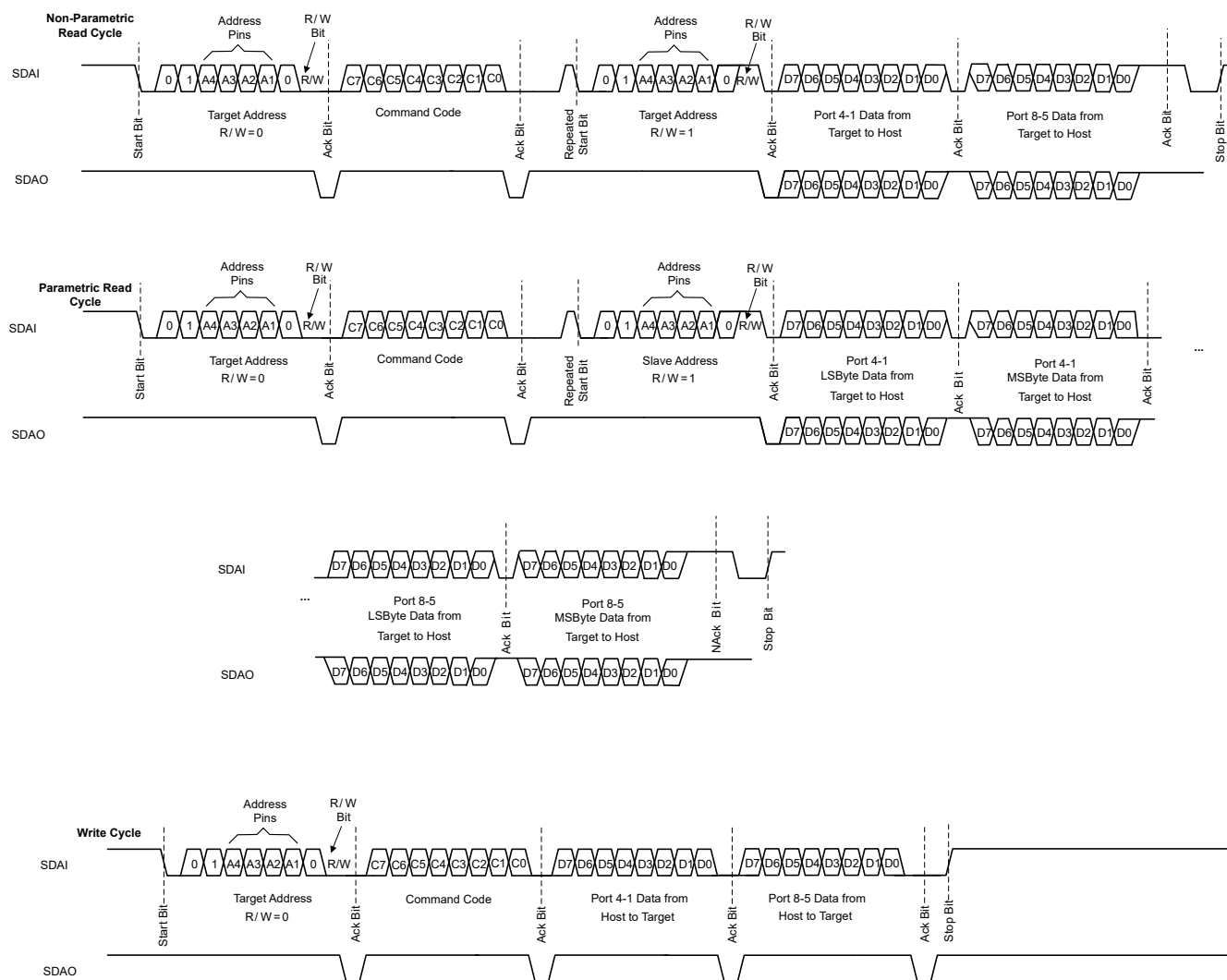
9-5. I 2 C interface Read and Write Protocol – Configuration B
