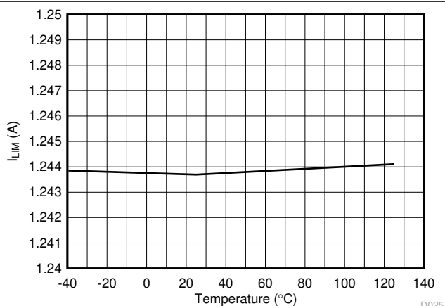
FIG 7-23. 2x Mode (2xFBn = 1) Current Limit vs Temperature
