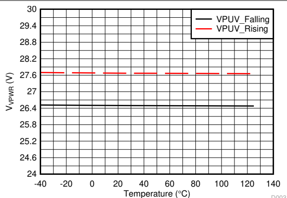
FIG 7-3. VPUV Thresholds vs Temperature
