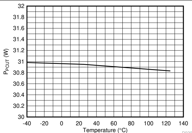
FIG 7-20. PCut Threshold (30W) vs Temperature
