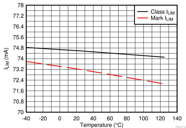
Figure 7-12. Classification and Mark Current Limit vs Temperature
