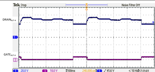
10-6. Semiauto Mode Discovery with a Valid Class 0-3 Load
