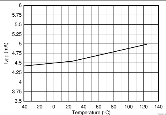
FIG 7-4. VDD Current Consumption vs Temperature
