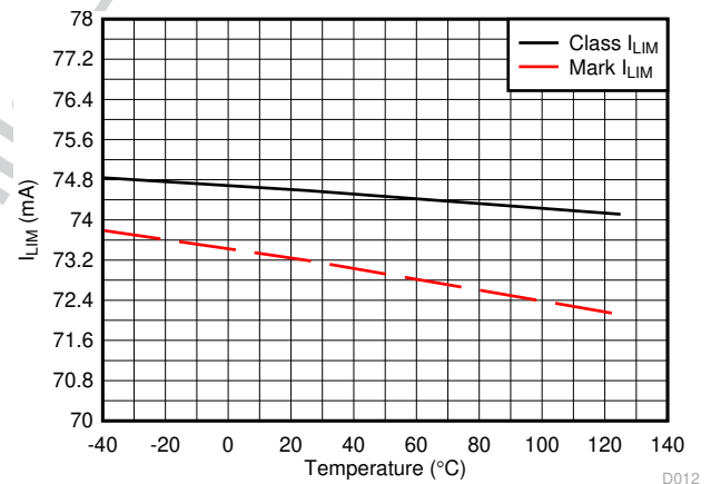
FIG 7-12. Classification and Mark Current Limit vs Temperature
