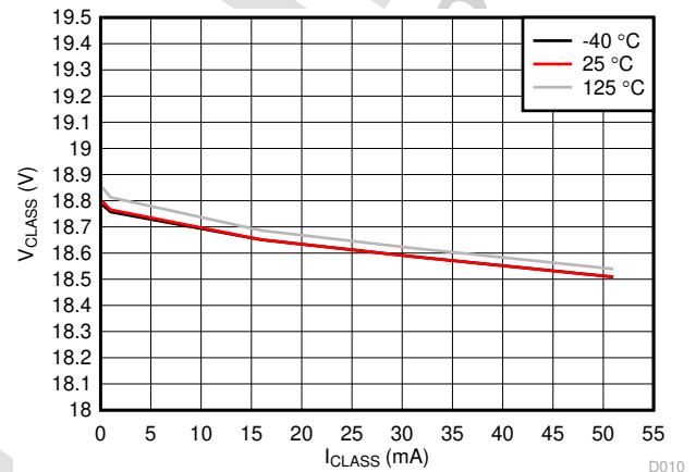
FIG 7-10. Classification Voltage vs I_{CLASS} and Temperature
