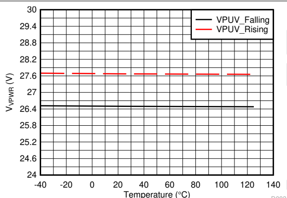
7-3. VPUV Thresholds vs Temperature
