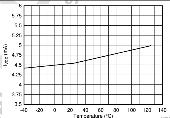
7-4. VDD Current Consumption vs Temperature
