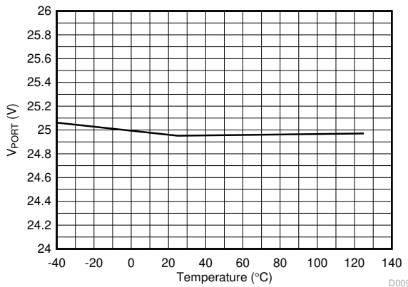
FIG 7-9. Discovery Open Circuit Voltage vs Temperature
