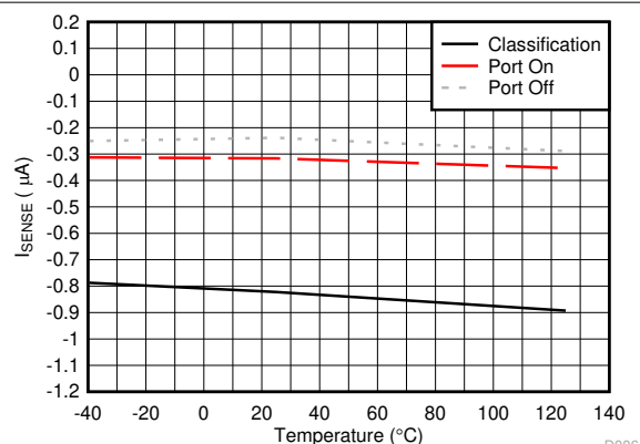
7-6. SENSE Pin Bias Current vs Temperature
