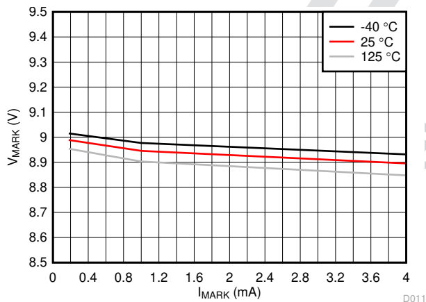
FIG 7-11. Mark Voltage vs I_{MARK} and Temperature
