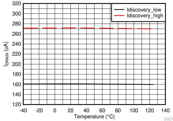
FIG 7-7. Discovery Currents vs Temperature
