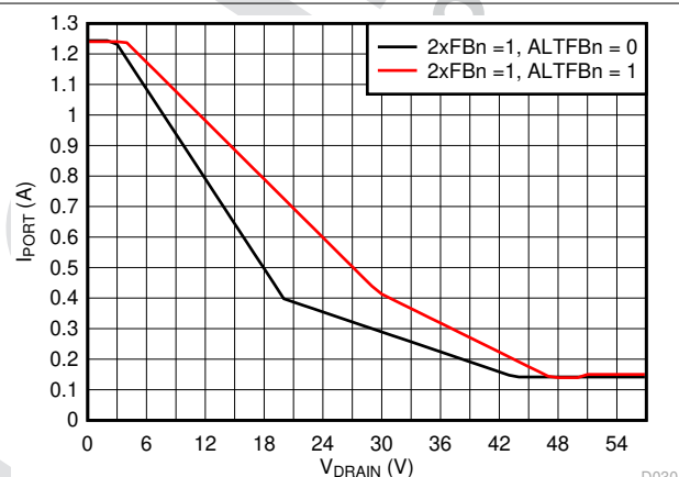
图 7-28. 2x Mode (2xFBn = 1) Current Foldback vs Drain Voltage
