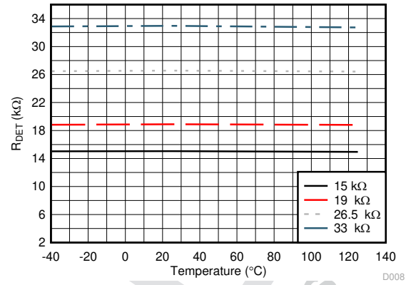
FIG 7-8. Discovery Resistance Measurement vs Temperature
