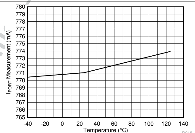
7-18. Port Current ADC Measurement (770mA) vs Temperature
