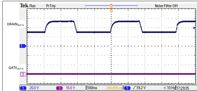
图 131. 2-Pair Open Circuit Detection Signature
