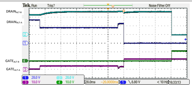
FIG 140. 4-Pair Single Signature 1-Finger Classification and Turn On
