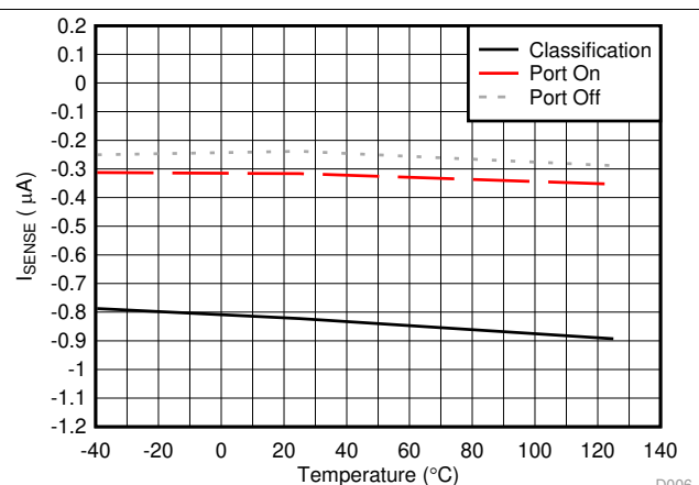
图 6. SENSE Pin Bias Current vs Temperature
