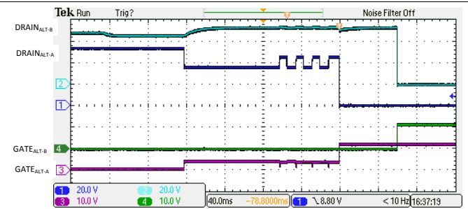
FIG 142. 4-Pair Single Signature 4-Finger Classification and Turn On
