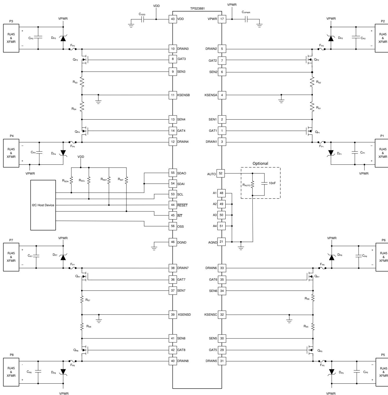
FIG 122. Eight 2-Pair Port Application
