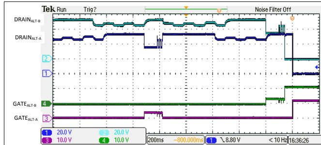
FIG 139. 4-Pair Single Signature Discovery and Turn On from Semi-Auto Mode
