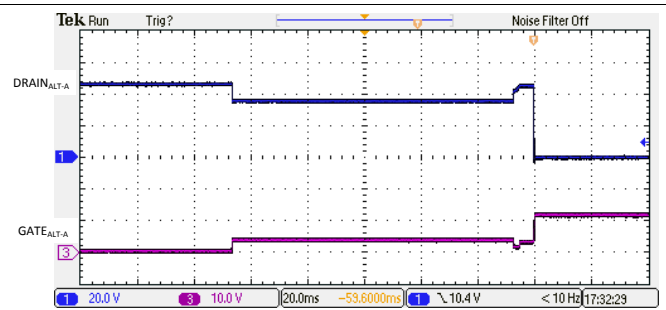
图 136. 2-Pair 1-Finger Classification and Turn On
