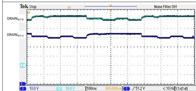
图 133. 4-Pair Low Resistance (11kΩ) Detection Signature
