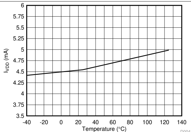
图 4. VDD Current Consumption vs Temperature
