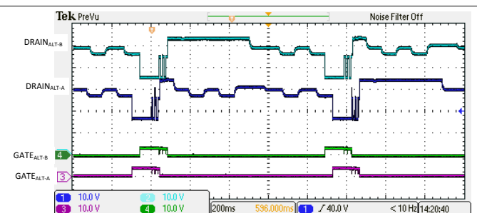
FIG 144. 4-Pair Semi-Auto Mode Discovery with a Valid Dual Signature Class 4D Load
