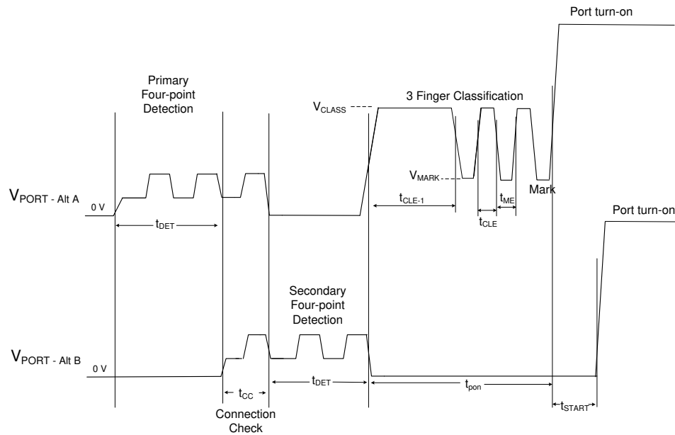
图 35. 4-Pair Single Signature Detection, 3-Event Classification and Turn On
