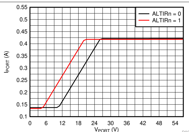
图 28. Inrush Current Foldback vs Port Voltage
