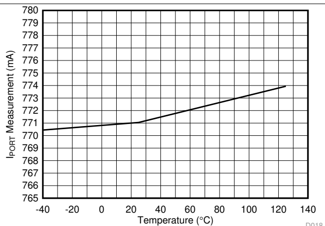
Figure 18. Port Current ADC Measurement (770mA) vs Temperature
