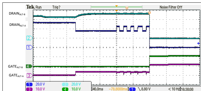
FIG 143. 4-Pair Single Signature 5-Finger Classification and Turn On
