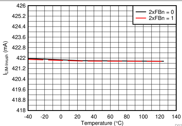
FIG 23. Inrush Current Limit vs Temperature
