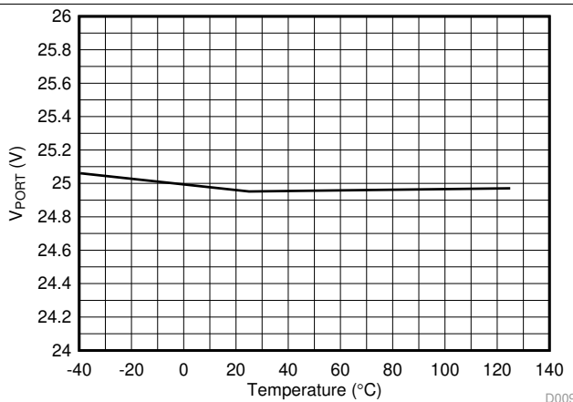
图 9. Discovery Open Circuit Voltage vs Temperature
