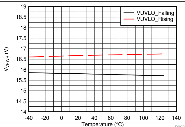
图 2. VPWR UVLO Thresholds vs Temperature
