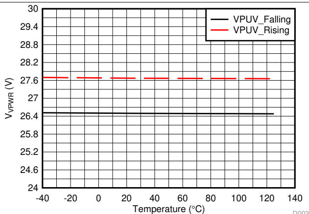
图 3. VPUV Thresholds vs Temperature
