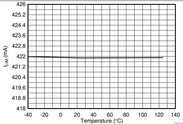
FIG 24. 1x Mode (2xFBn = 0) Current Limit vs Temperature
