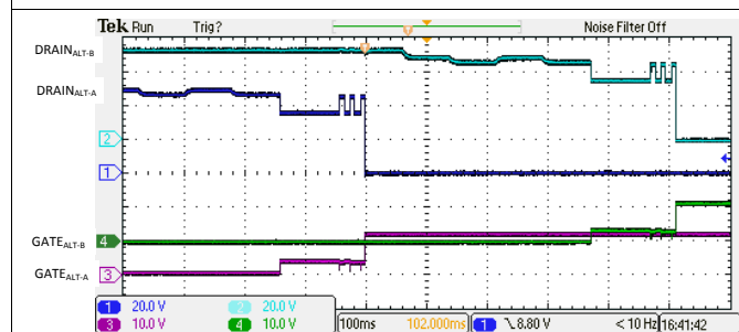
FIG 147. 4-Pair Dual Signature 3-Finger Classification and Turn On
