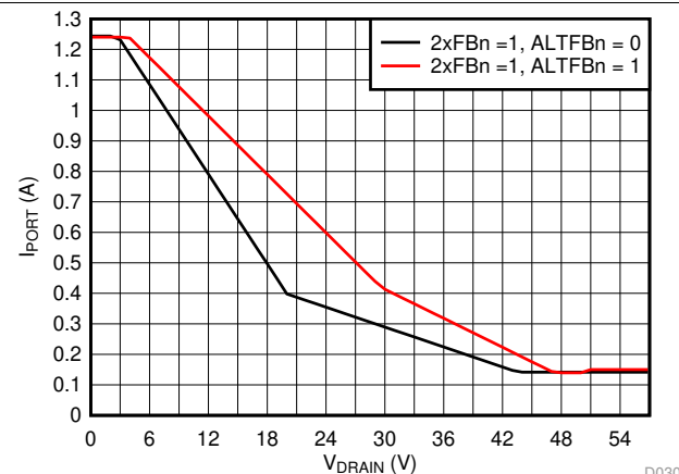
图 30. 2x Mode (2xFBn = 1) Current Foldback vs Drain Voltage
