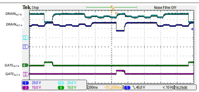
图 138. 4-Pair Semi-Auto Mode Discovery with a Valid Single Signature Class 0-3 Load
