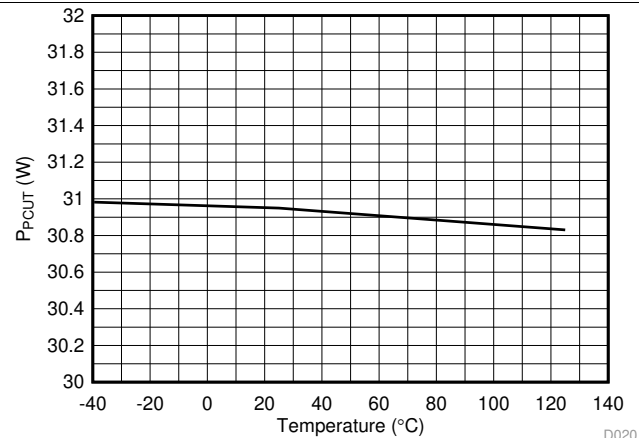
FIG 20. 2-Pair PCut Threshold (30W) vs Temperature
