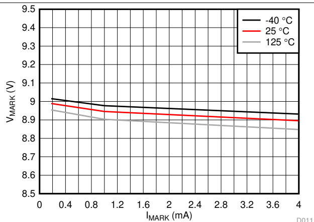
图 11. Mark Voltage vs I_{MARK} and Temperature
