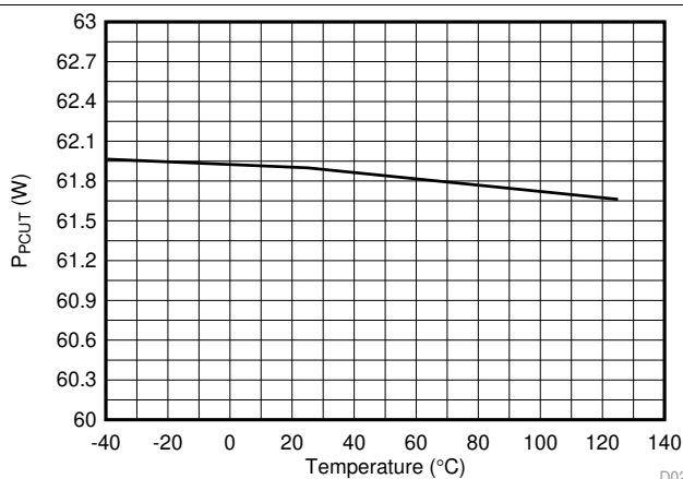
FIG 21. 4-Pair PCut Threshold (60W) vs Temperature
