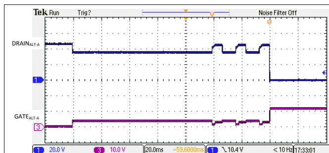
图 137. 2-Pair 3-Finger Classification and Turn On
