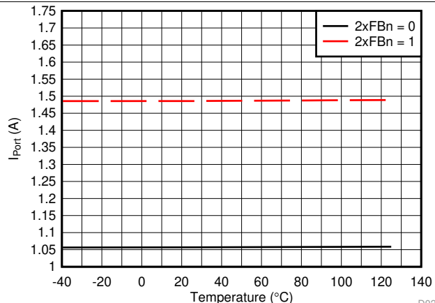
图 26. I_SHORT Threshold vs Temperature
