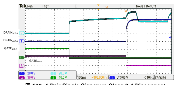
图 130. 4-Pair Single Signature Class 0-4 Disconnect
