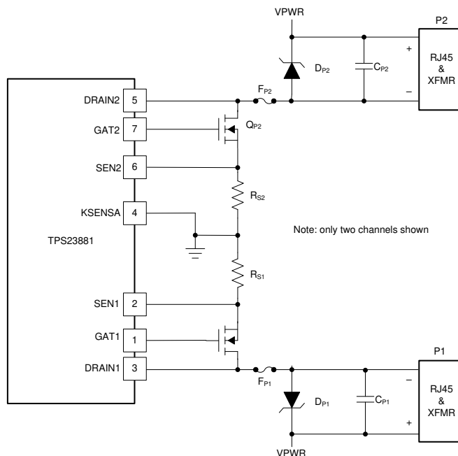
FIG 149. Kelvin Current-Sense Connection
