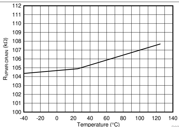
图 27. R_OFF (VPWR to DRAIN) vs Temperature
