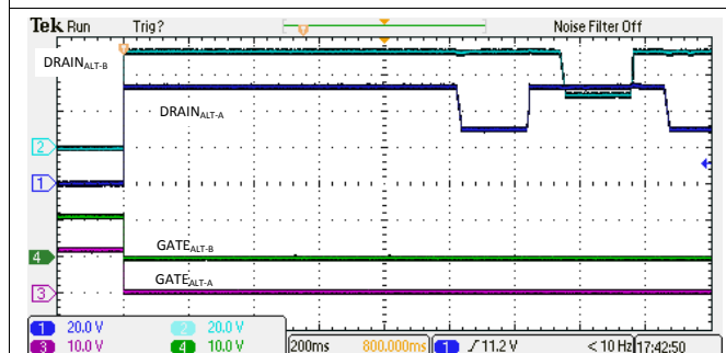
图 129. 4-Pair Backoff Due to 4PPCut Fault
