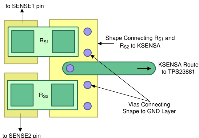
FIG 150. Kelvin Sense Layout Example
