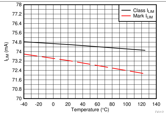
图 12. Classification and Mark Current Limit vs Temperature
