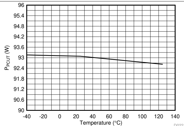
FIG 22. 4-Pair PCut Threshold (90W) vs Temperature
