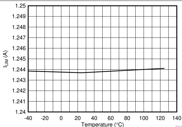
图 25. 2x Mode (2xFBn = 1) Current Limit vs Temperature
