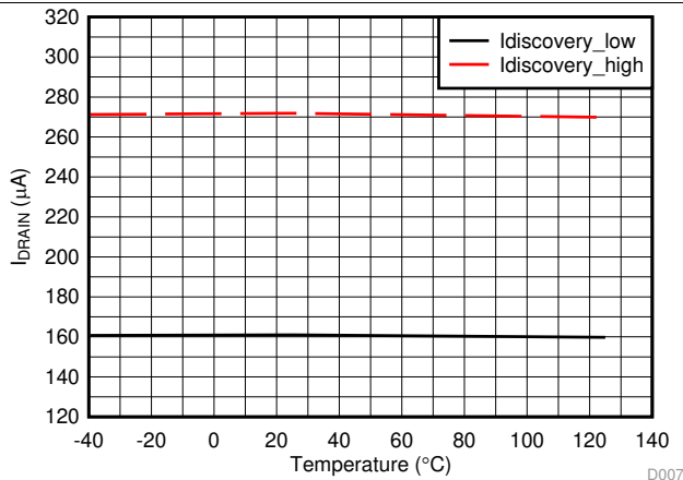
图 7. Discovery Currents vs Temperature
