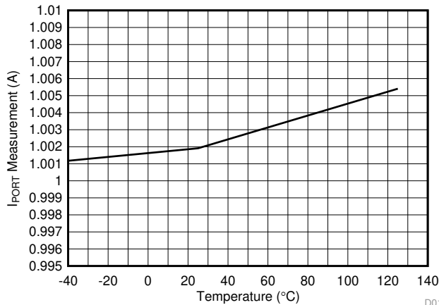
FIG 19. Port Current ADC Measurement (1 A) vs Temperature
