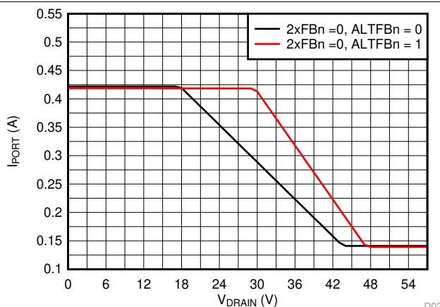
图 29. 1x Mode (2xFBn = 0) Current Foldback vs Drain Voltage
