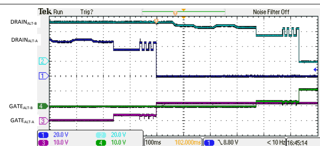
FIG 148. 4-Pair Dual Signature 4-Finger Classification and Turn On
