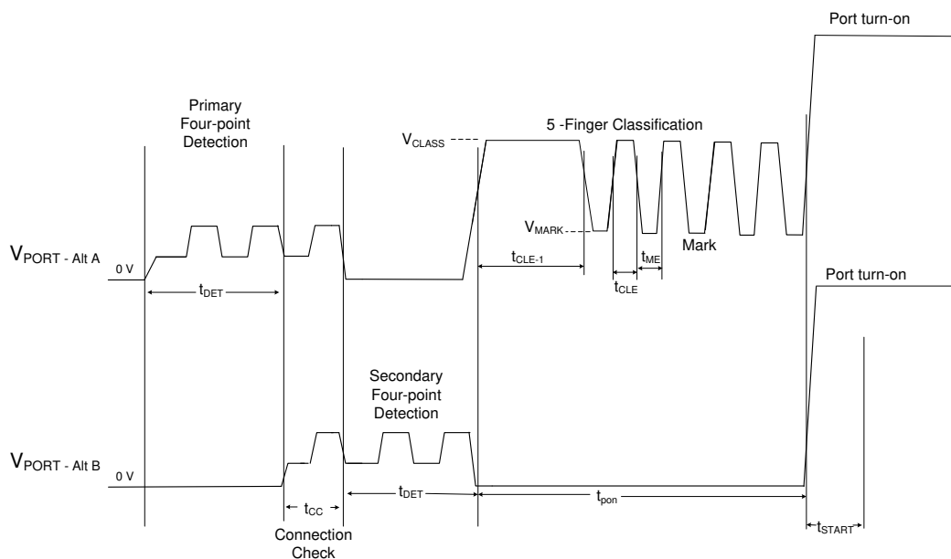
图 36. 4-Pair Single Signature Detection, 5-Event Classification and Turn On
