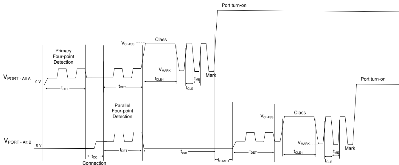
37. 4-Pair Dual Signature Detection, 3-Event Classification and Turn On
