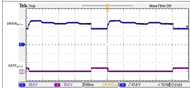
图 135. 2-Pair Semi-Auto Mode Discovery with a Valid Class 0-3 Load
