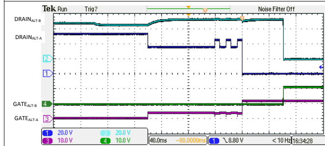
FIG 141. 4-Pair Single Signature 3-Finger Classification and Turn On
