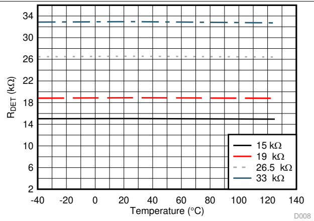
图 8. Discovery Resistance Measurement vs Temperature
