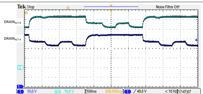
图 134. 4-Pair High Resistance (36kΩ) Detection Signature
