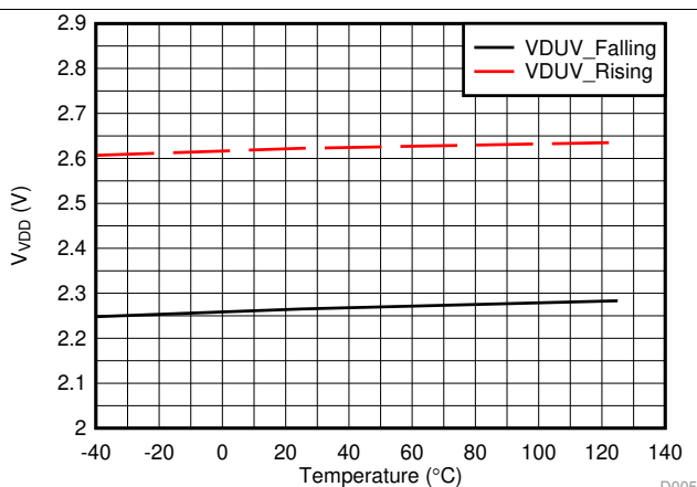
图 5. VDUV Thresholds vs Temperature
