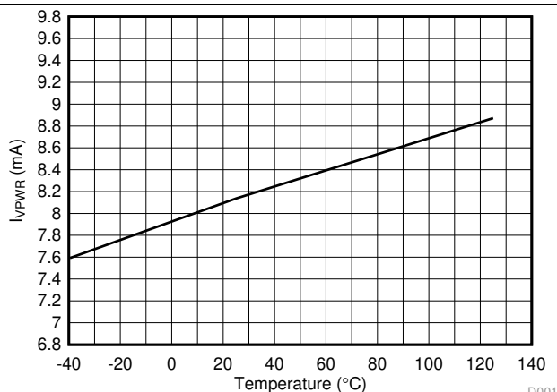
图 1. VPWR Current Consumption vs Temperature
