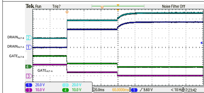
图 127. 4-Pair I_{LIM} Foldback and Turn Off
