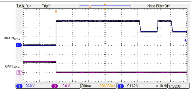
图 126. 2-Pair Backoff due to PCut Fault
