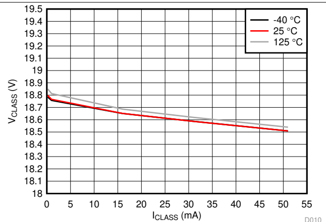
图 10. Classification Voltage vs I_{CLASS} and Temperature
