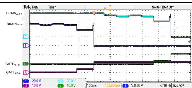
FIG 146. 4-Pair Dual Signature 1-Finger Classification and Turn On
