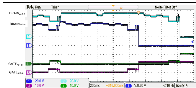
FIG 145. 4-Pair Dual Signature Discovery and Turn On from Semi-Auto Mode
