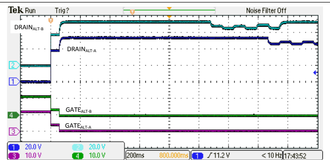
图 128. 4-Pair Backoff Due to I_{LIM} Fault
