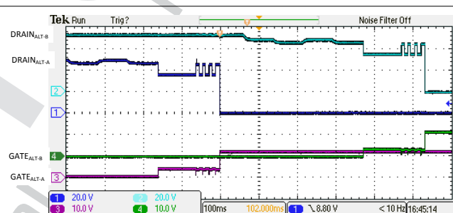
10-27. 4-Pair Dual Signature 4-Finger Classification and Turn On
