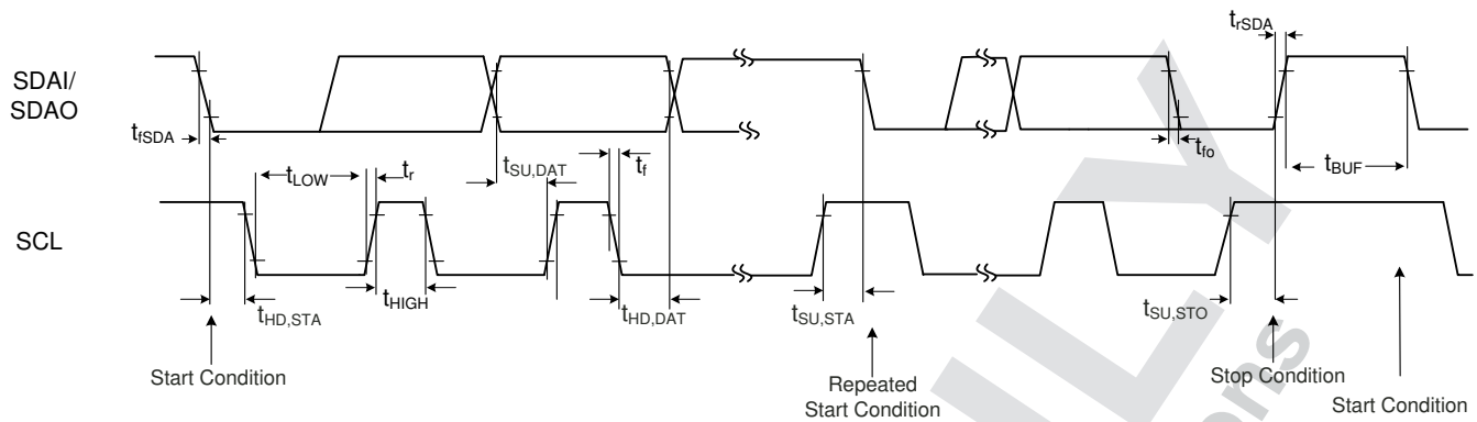
FIG 8-1. I 2 C Timings
