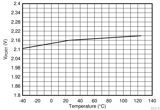
7-13. Power Good Threshold vs Temperature
