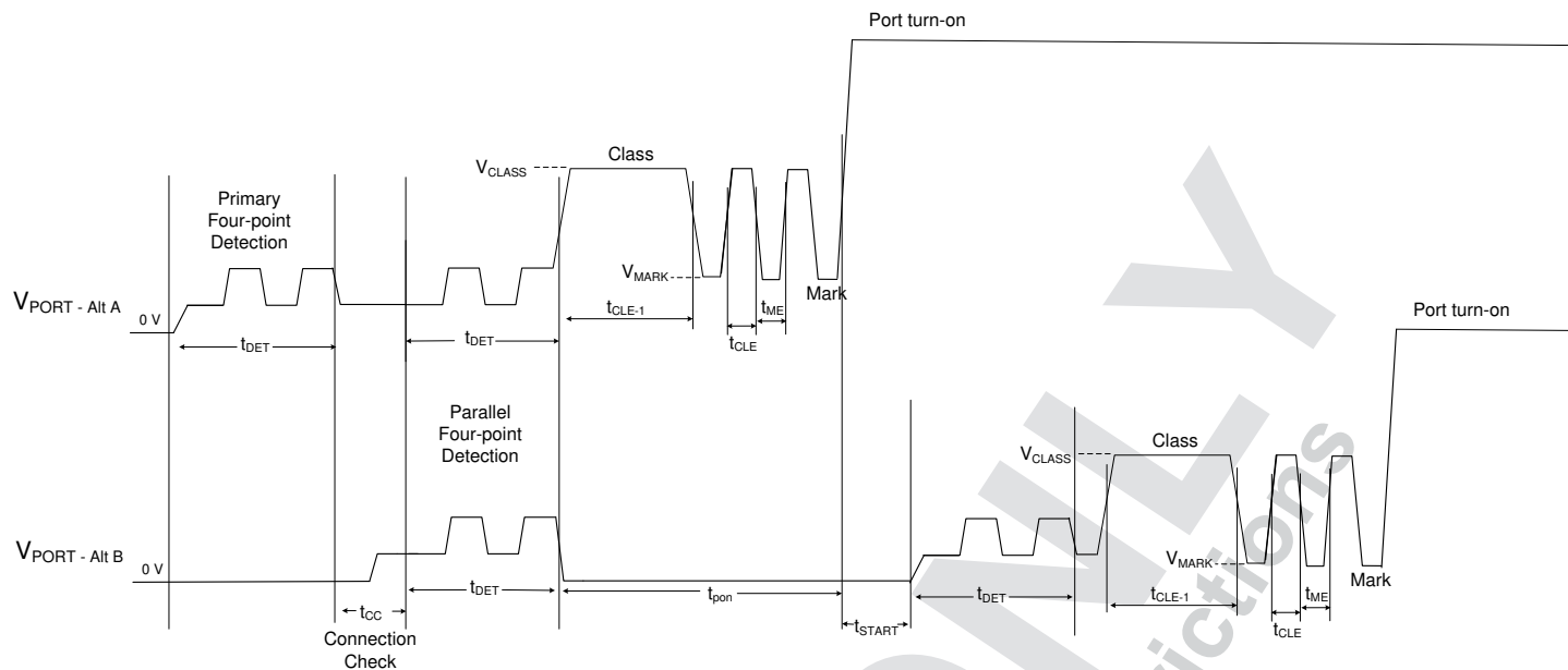
8-7. 4-Pair Dual Signature Detection, 3-Event Classification and Turn On
