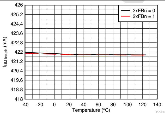
7-23. Inrush Current Limit vs Temperature
