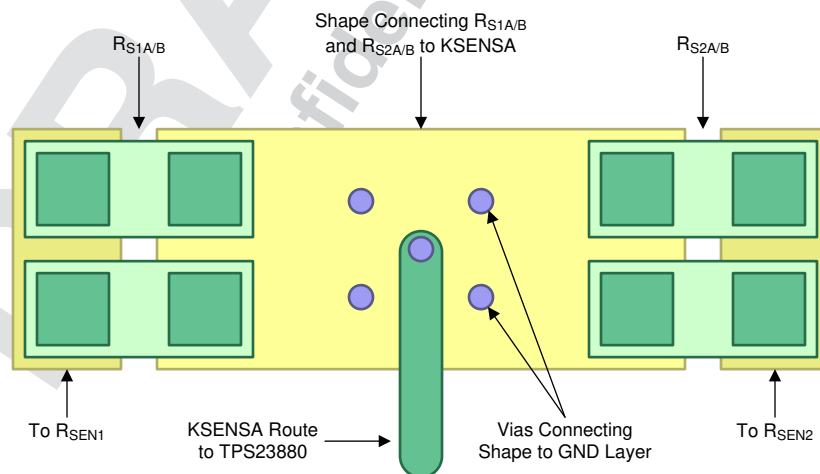
FIG 12-2. Kelvin Sense Layout Example
