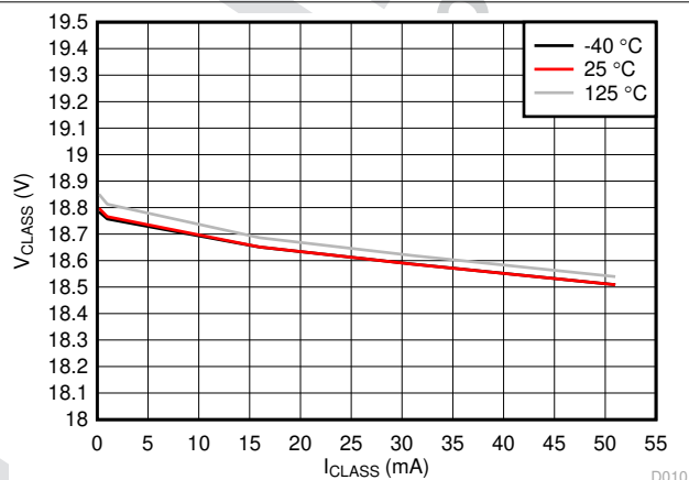
7-10. Classification Voltage vs I_{CLASS} and Temperature
