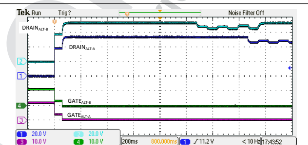
FIG 10-7. 4-Pair Backoff Due to I_{LIM} Fault
