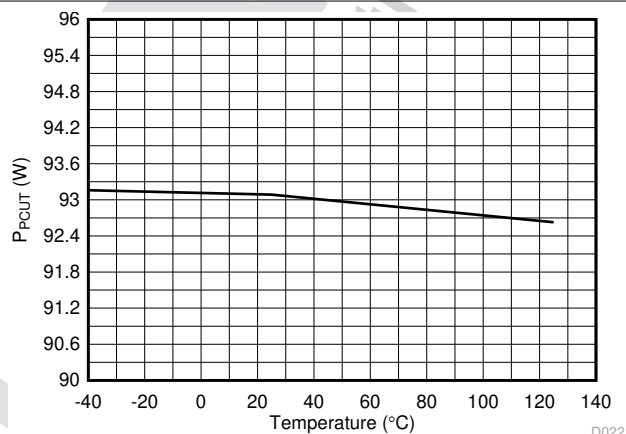
7-22. 4-Pair PCut Threshold (90W) vs Temperature
