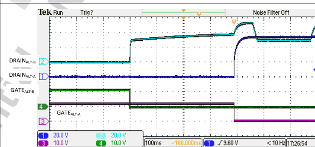
10-9. 4-Pair Single Signature Class 0-4 Disconnect
