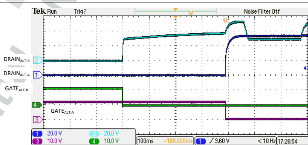
FIG 10-9. 4-Pair Single Signature Class 0-4 Disconnect
