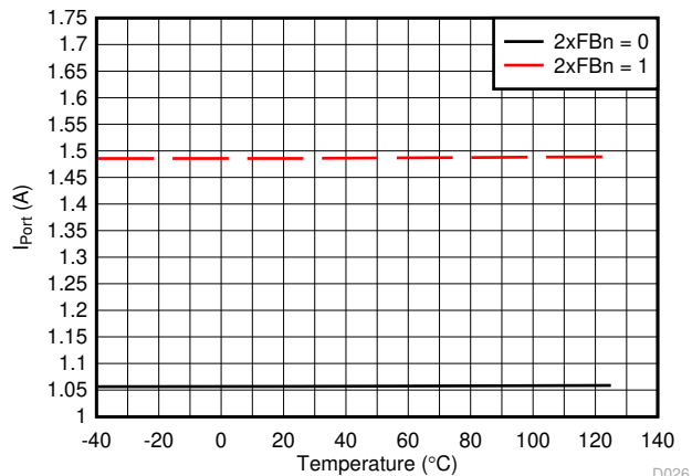
7-26. I_{SHORT} Threshold vs Temperature
