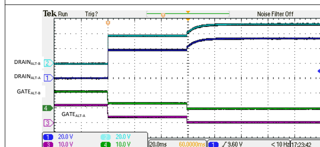
10-6. 4-Pair I_{LIM} Foldback and Turn Off
