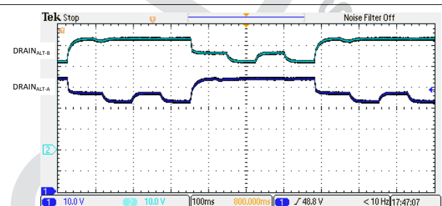
10-13. 4-Pair High Resistance (36kΩ) Detection Signature
