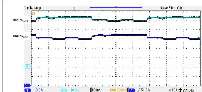
10-12. 4-Pair Low Resistance (11kΩ) Detection Signature
