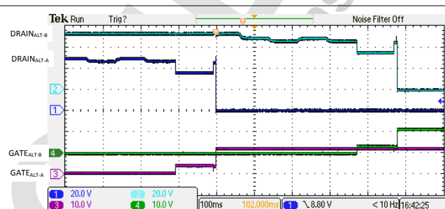
10-25. 4-Pair Dual Signature 1-Finger Classification and Turn On
