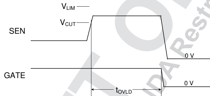
FIG 8-2. Overcurrent Fault Timing
