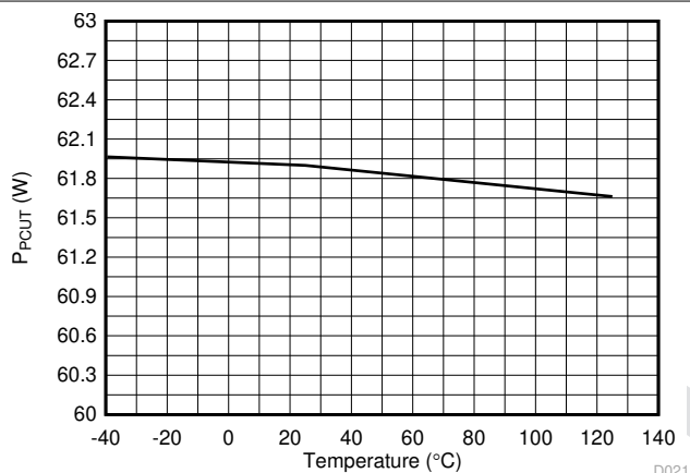
7-21. 4-Pair PCut Threshold (60W) vs Temperature
