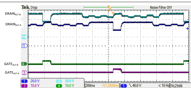
10-17. 4-Pair Semi-Auto Mode Discovery with a Valid Single Signature Class 0-3 Load
