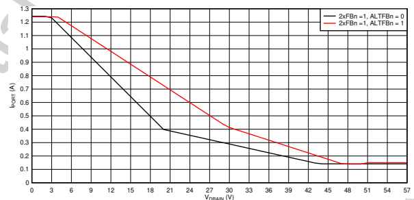
图 9-56. 2x Mode (2xFBn = 1) Foldback Curves, I_{PORT} vs V_{DRAIN}
