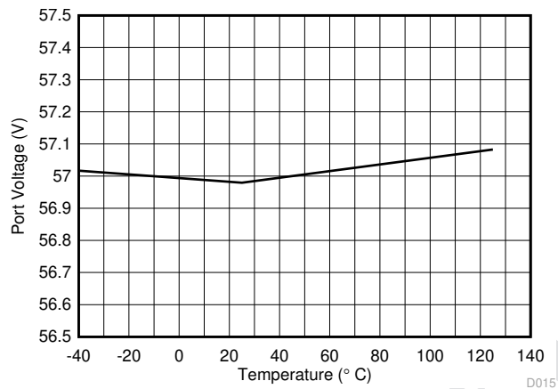
7-15. Port Voltage ADC Measurement vs Temperature
