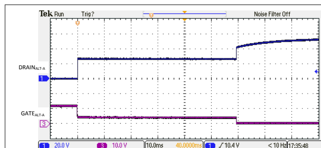
10-4. 2-Pair I_{LIM} Foldback and Turn Off
