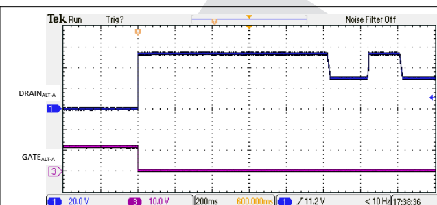
10-5. 2-Pair Backoff due to PCut Fault
