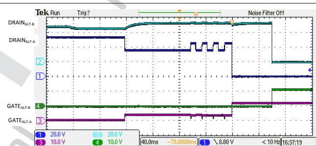
10-21. 4-Pair Single Signature 4-Finger Classification and Turn On
