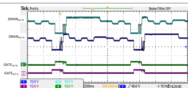
10-23. 4-Pair Semi-Auto Mode Discovery with a Valid Dual Signature Class 4D Load
