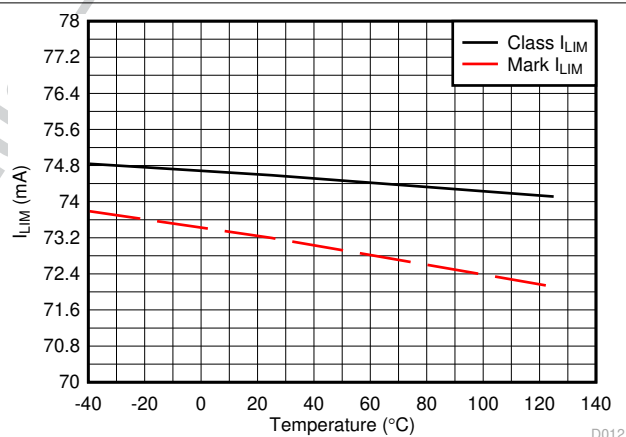
7-12. Classification and Mark Current Limit vs Temperature
