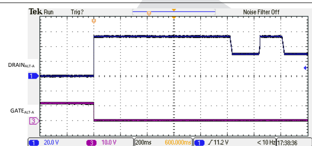
FIG 10-5. 2-Pair Backoff due to PCut Fault
