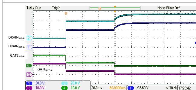
FIG 10-6. 4-Pair I_{LIM} Foldback and Turn Off
