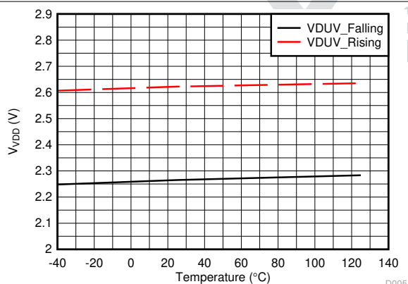
7-5. VDUV Thresholds vs Temperature
