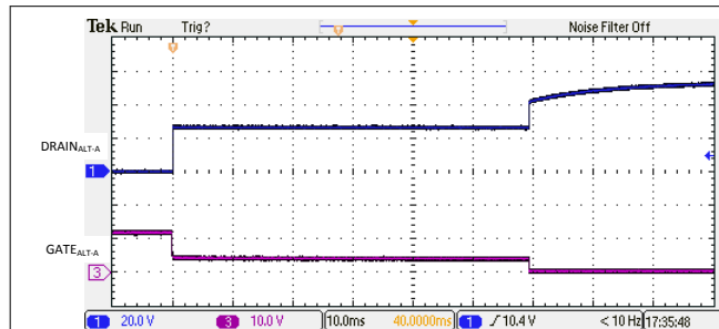
FIG 10-4. 2-Pair I_{LIM} Foldback and Turn Off
