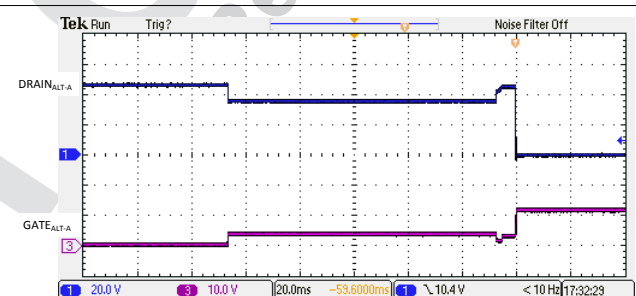
10-15. 2-Pair 1-Finger Classification and Turn On
