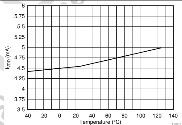
7-4. VDD Current Consumption vs Temperature
