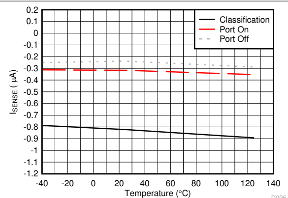
7-6. SENSE Pin Bias Current vs Temperature
