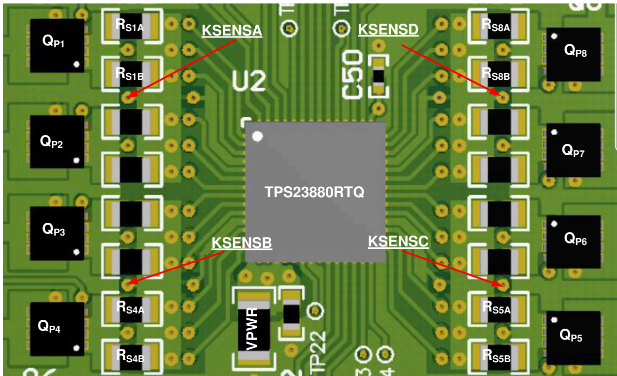
FIG 12-3. Eight Port Layout Example (Top Side)
