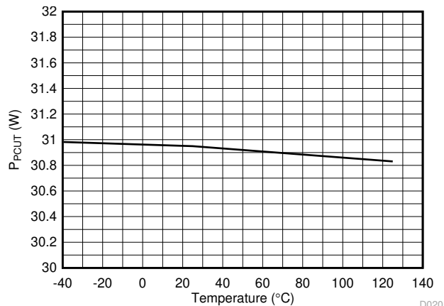
7-20. 2-Pair PCut Threshold (30W) vs Temperature
