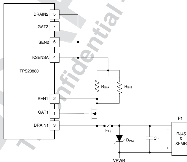
図 10-3. Unused PORT2 Connections
