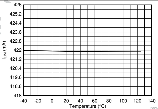
7-24. 1x Mode (2xFBn = 0) Current Limit vs Temperature
