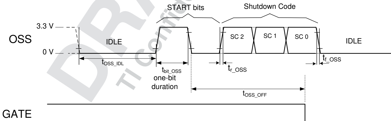
Figure 9-1. Multi Bit Priority Port Shutdown if Lower-Priority Port
