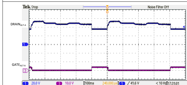
10-14. 2-Pair Semi-Auto Mode Discovery with a Valid Class 0-3 Load
