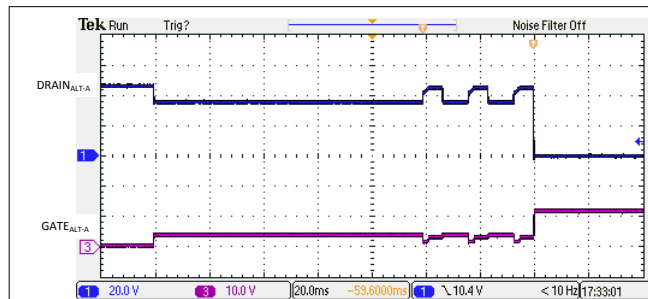
10-16. 2-Pair 3-Finger Classification and Turn On
