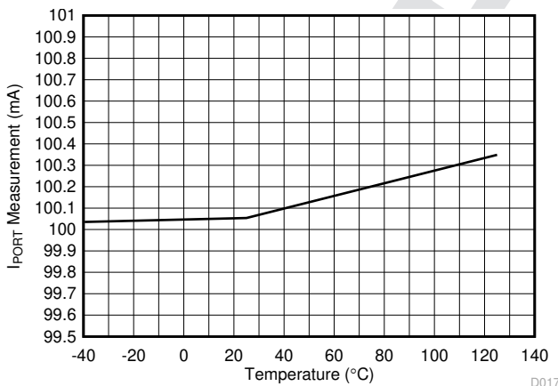
7-17. Port Current ADC Measurement (100mA) vs Temperature
