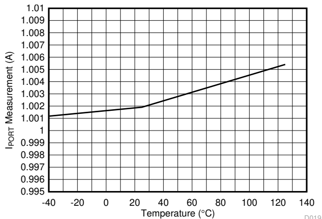
7-19. Port Current ADC Measurement (1 A) vs Temperature
