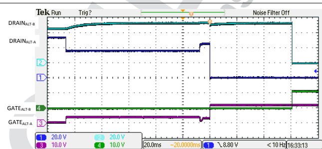
10-19. 4-Pair Single Signature 1-Finger Classification and Turn On
