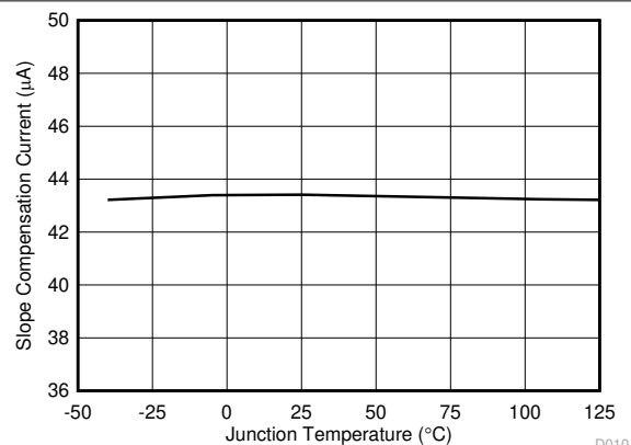
6-14. Current Slope Compensation Current vs Temperature
