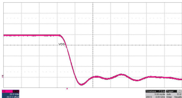
8-8. Slew Rate Adjust SRF = 0 \Omega
