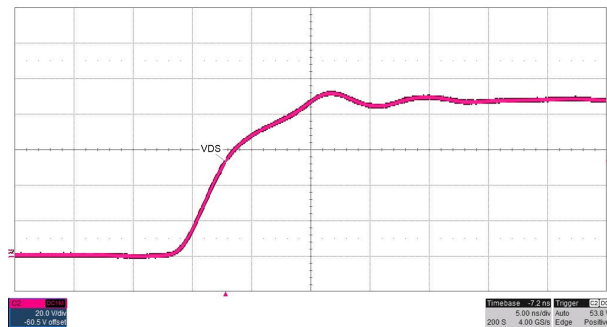
8-7. Slew Rate Adjust SRR = 0 \Omega
