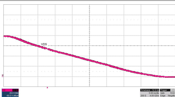
8-10. Slew Rate Adjust SRF = 100 \Omega
