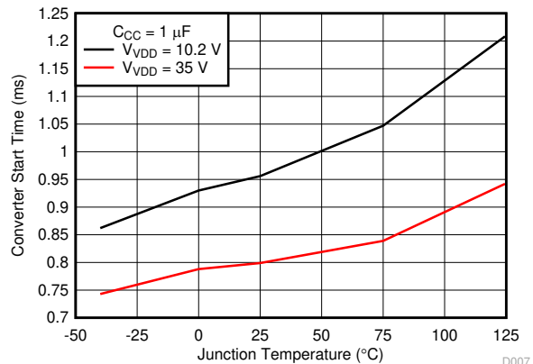
FIG 6-6. Converter Startup Time vs Temperature
