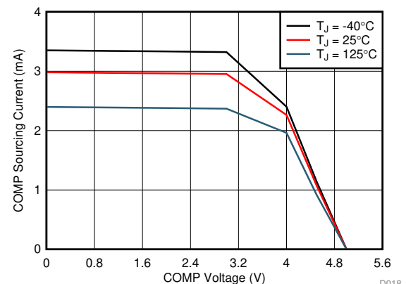
6-18. Error Amplifier Source Current
