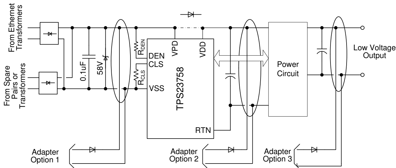
7-10. ORing Configurations
