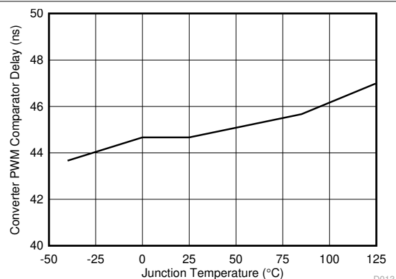
6-16. Converter PWM Comparator Delay vs Temperature
