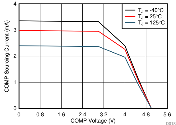
FIG 6-19. Error Amplifier Source Current
