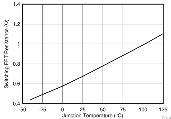
FIG 6-23. Switching FET Resistance vs Temperature
