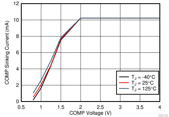
FIG 6-20. Error Amplifier Sink Current
