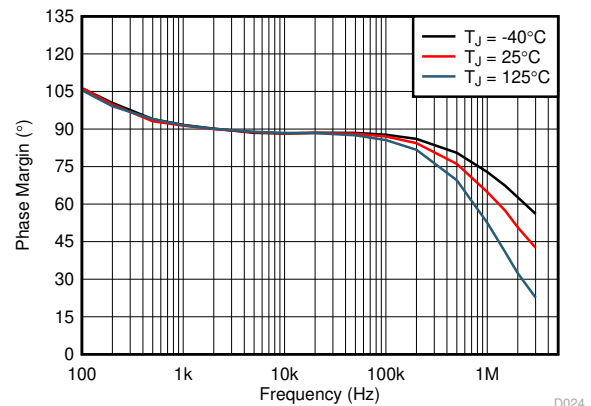
FIG 6-22. Error Amplifier Phase vs Frequency
