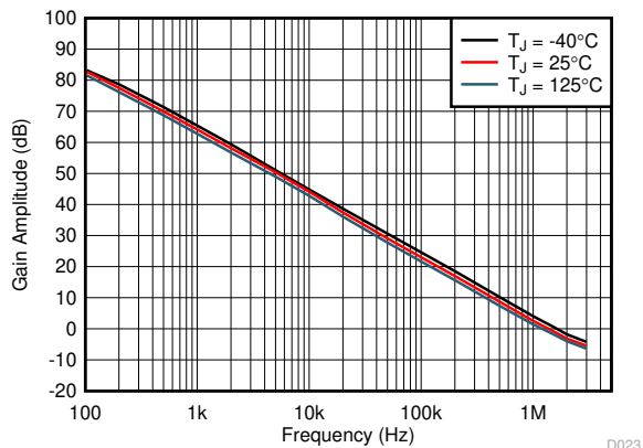
FIG 6-21. Error Amplifier Gain vs Frequency
