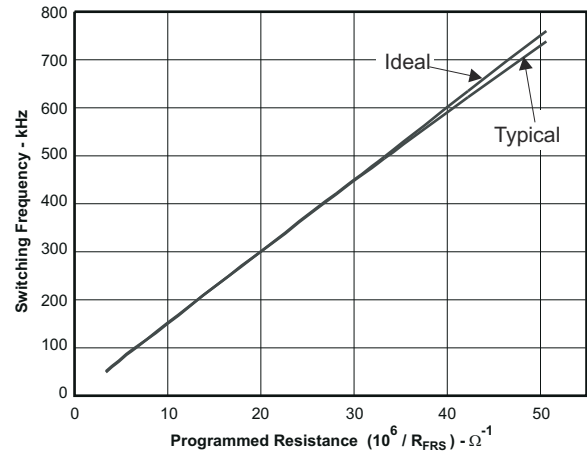
Figure 7-8. Switching Frequency vs Programmed Resistance
