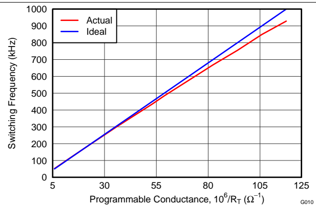
Figure 13. Switching Frequency vs Programmable Conductance
