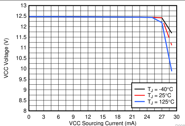
7-7. Converter Startup Voltage vs Current
