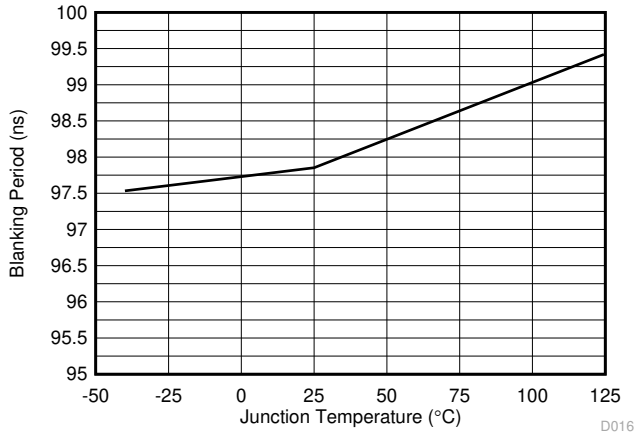
7-15. Blanking Period vs Temperature
