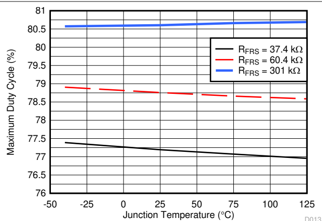
7-12. Maximum Duty Cycle vs Temperature
