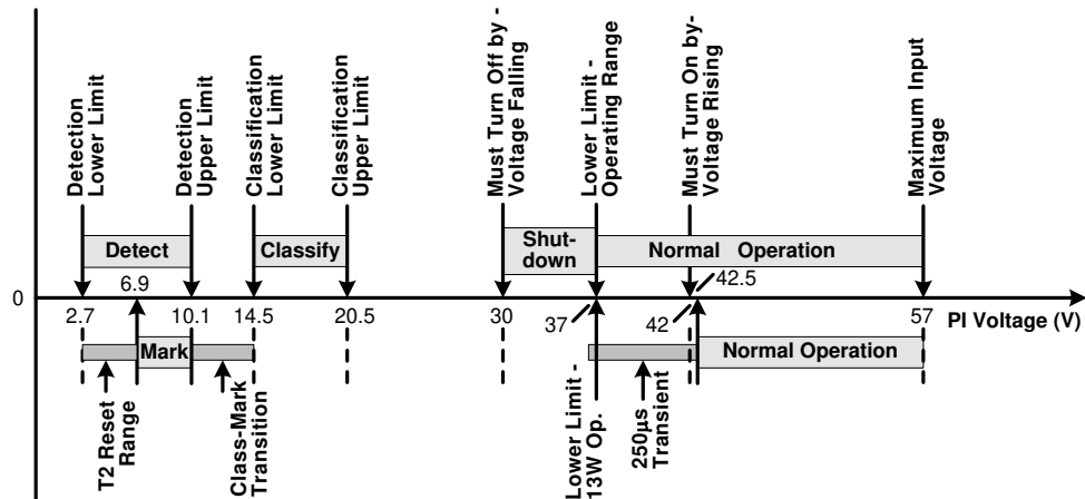
图 8-5. Operational States
