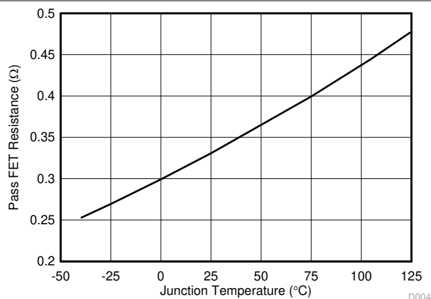
7-3. Pass FET Resistance vs Temperature
