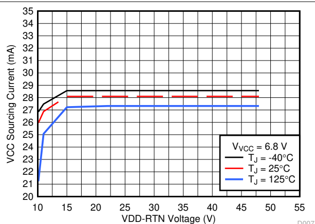
7-6. Converter Startup Current vs VDD Input Voltage
