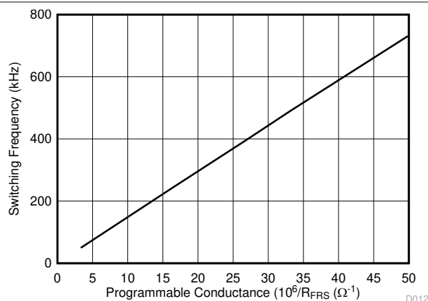
7-11. Switching Frequency vs Programmed Resistance
