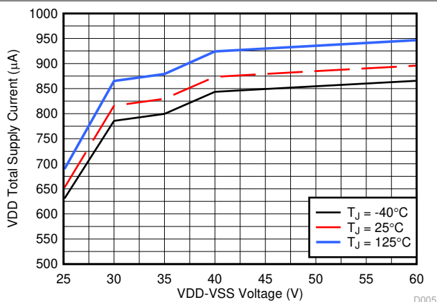
7-4. VDD Supply Current vs Voltage
