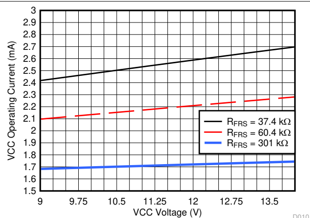
7-9. Controller Bias Current vs Voltage
