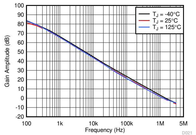
7-18. Error Amplifier Gain vs Frequency
