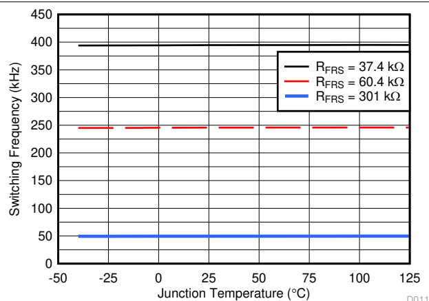
7-10. Switching Frequency vs Temperature
