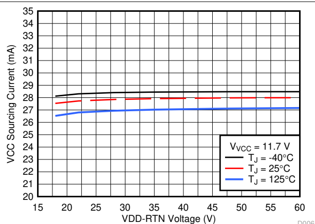
7-5. Converter Startup Current vs VDD Input Voltage
