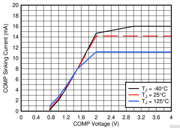
7-17. Error Amplifier Sink Current
