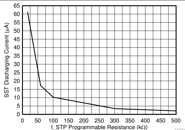
7-8. Controller SST Soft Stop Sink Current vs Programmed Resistance
