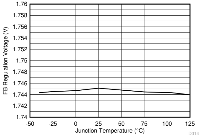
7-13. Feedback Regulation Voltage vs Temperature
