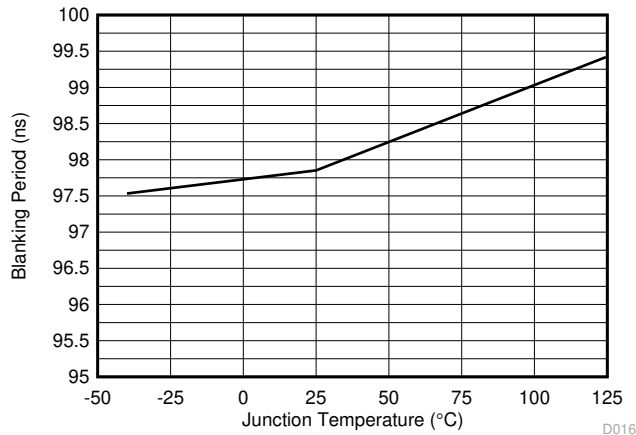
FIG 7-16. Blanking Period vs Temperature
