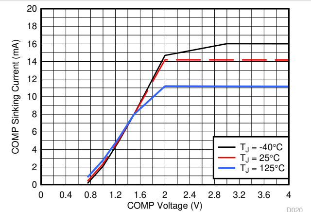
FIG 7-19. Error Amplifier Sink Current
