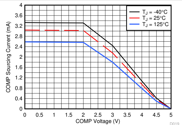
FIG 7-18. Error Amplifier Source Current
