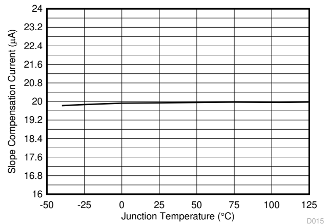
FIG 7-15. Current Slope Compensation Current vs Temperature
