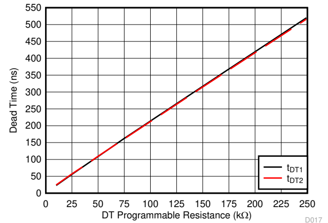
FIG 7-17. Dead Time vs Dead Time Resistance ( R_{DT} )
