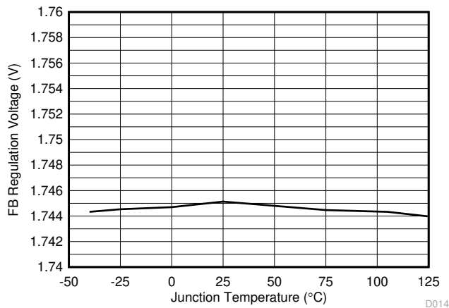
FIG 7-14. Feedback Regulation Voltage vs Temperature
