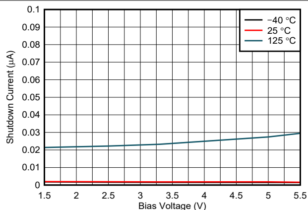
Figure 6-2. Shutdown Current vs Bias Voltage
