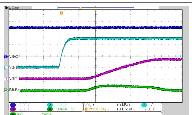
図 9-7. Inrush Current With CT = 220 pF
