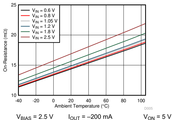
図 6-11. On-Resistance vs Ambient Temperature Single Channel (TPS22976A, TPS22976N)
