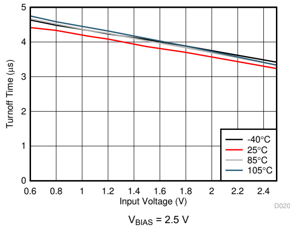
6-25. Turnoff Time vs Input Voltage (TPS22976N)
