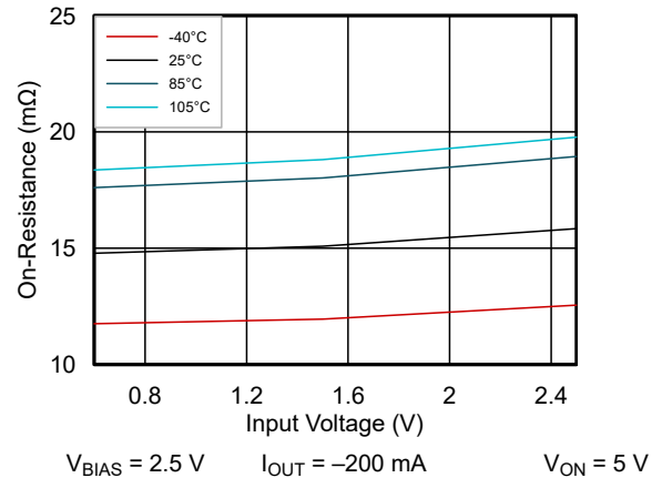
図 6-8. On-Resistance vs Input Voltage Single Channel - Across Ambient Temperatures (TPS22976)
