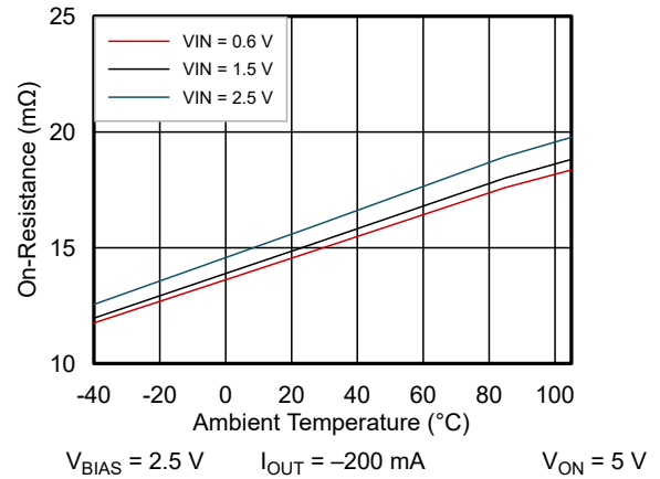
図 6-10. On-Resistance vs Ambient Temperature Single Channel (TPS22976)
