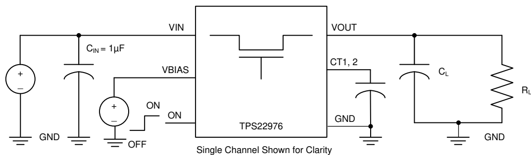
7-1. Test Circuit
