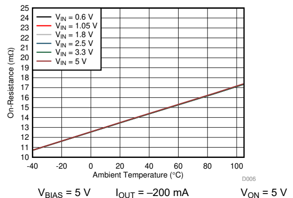
図 6-12. On-Resistance vs Ambient Temperature Single Channel (TPS22976A, TPS22976N)
