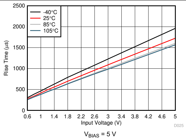
6-30. Rise Time vs Input Voltage
