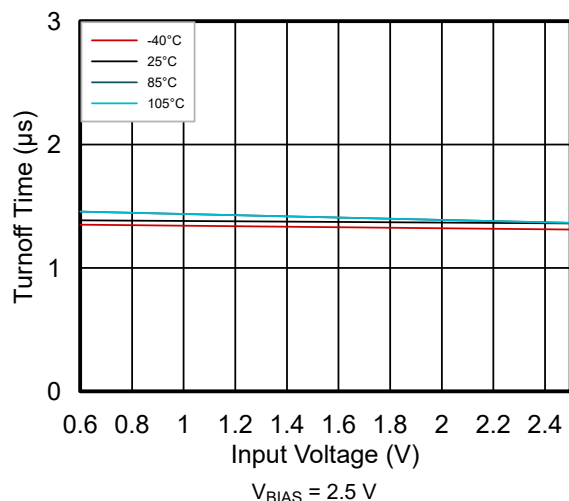
図 6-23. Turnoff Time vs Input Voltage (TPS22976)
