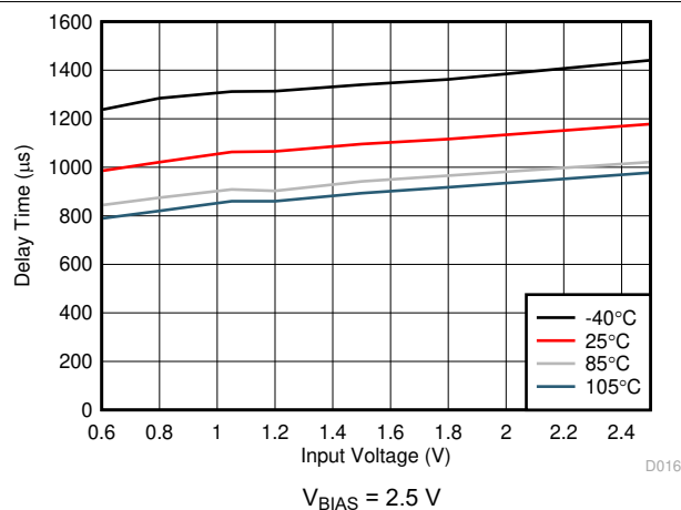
図 6-19. Delay Time vs Input Voltage
