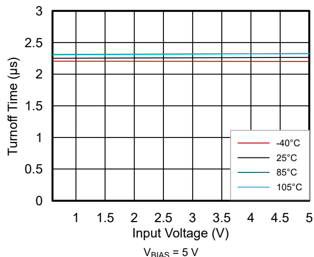
図 6-24. Turnoff Time vs Input Voltage (TPS22976)
