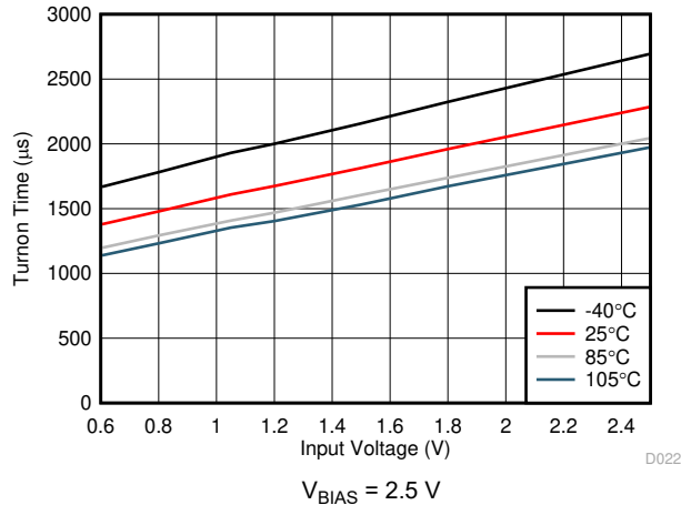
6-27. Turnon Time vs Input Voltage
