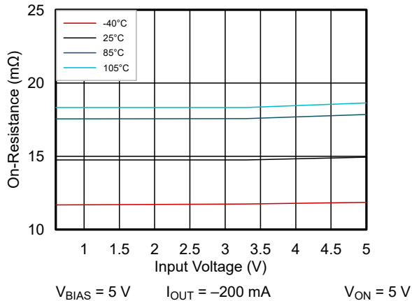
図 6-7. On-Resistance vs Input Voltage Single Channel - Across Ambient Temperatures (TPS22976)
