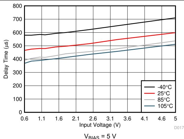
図 6-20. Delay Time vs Input Voltage
