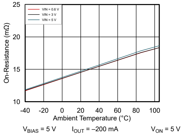
図 6-9. On-Resistance vs Ambient Temperature Single Channel (TPS22976)
