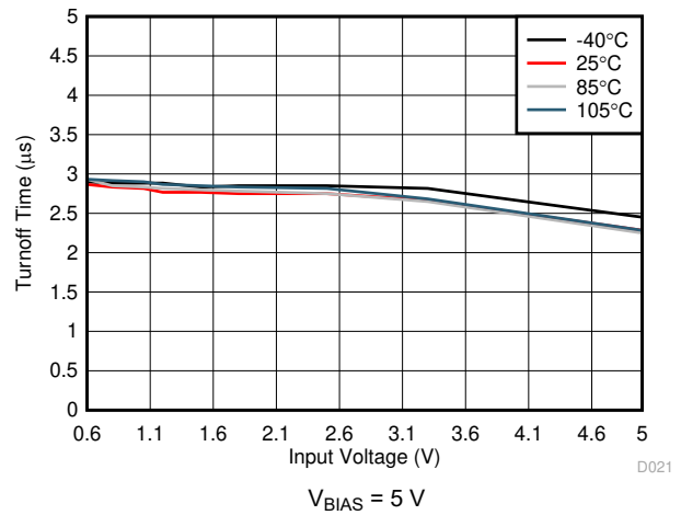
6-26. Turnoff Time vs Input Voltage (TPS22976N)
