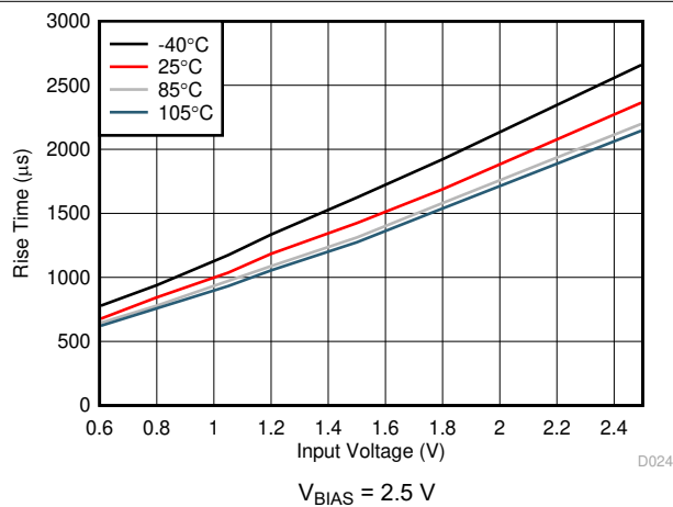
6-29. Rise Time vs Input Voltage
