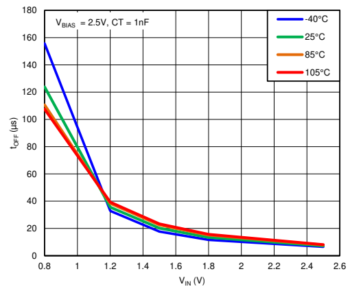
FIG 16. t_{OFF} vs. V_{IN} ( V_{BIAS} = 2.5\text{ V} , C_T = 1\text{ nF} )
