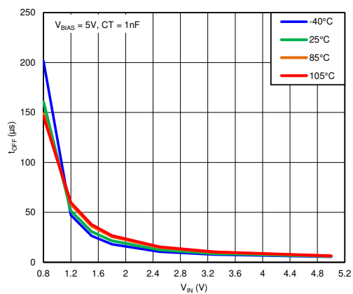
FIG 17. t_{OFF} vs. V_{IN} ( V_{BIAS} = 5\text{ V} , C_T = 1\text{ nF} )
