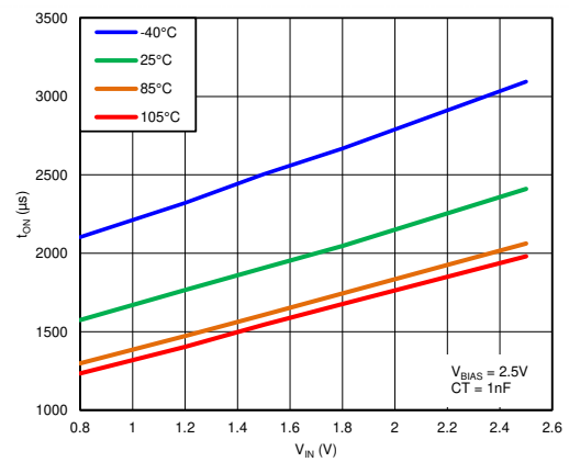
FIG 18. t_{ON} vs. V_{IN} ( V_{BIAS} = 2.5\text{ V} , C_T = 1\text{ nF} )
