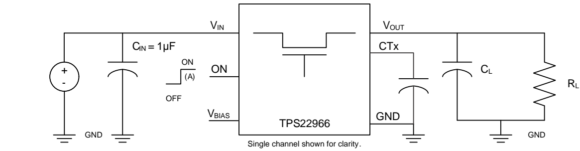
Test Circuit
