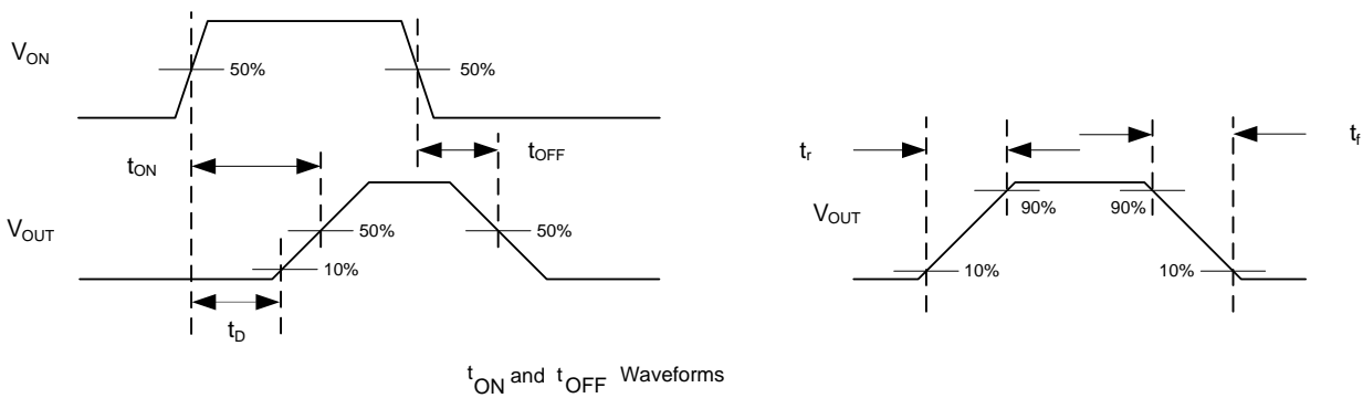
Figure 31. Test Circuit and t_{ON} - t_{OFF} Waveforms
