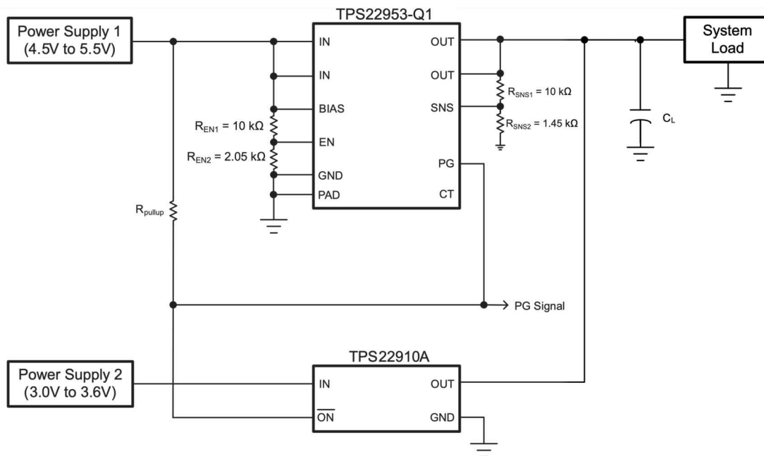
10-5. Make-Before-Break Power MUX Schematic
