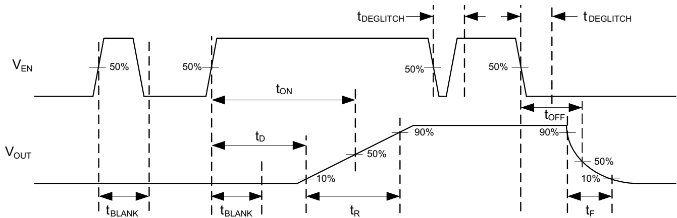
图 8-2. Timing Waveforms
