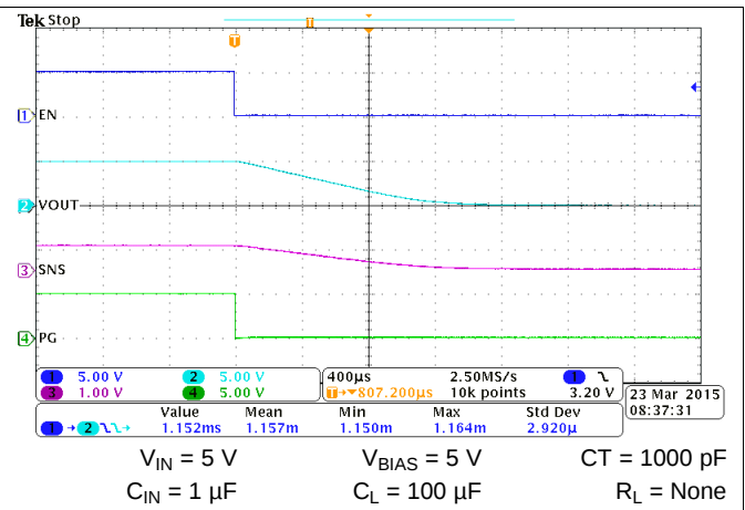
Figure 49. Quick Output Discharge of 100-µF Load ( t_{DIS} )
