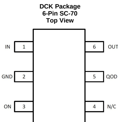
Pin Functions
