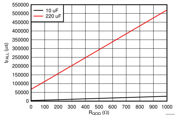
图 7-28. Turn-Off Time (Open Load)
