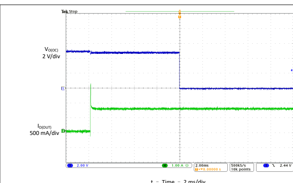
図 6-18. 2-Ω Load Connected to Enabled Device
