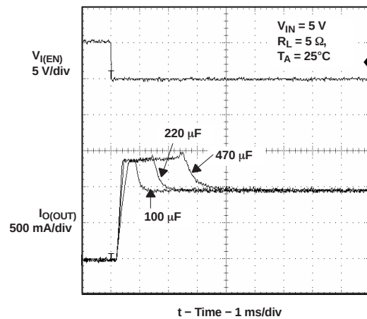
Figure 20. Inrush Current With Different Load Capacitance
