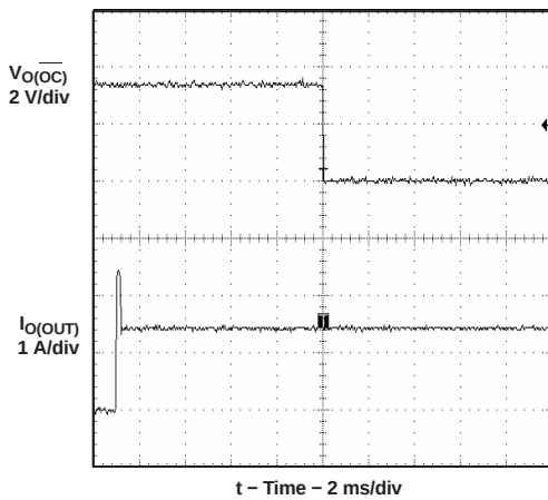
Figure 21. 2- \Omega Load Connected to Enabled Device
