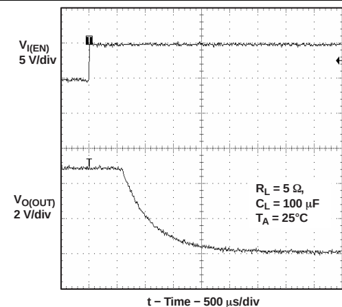
Figure 18. Turnoff Delay and Fall Time With 100- \mu\text{F} Load
