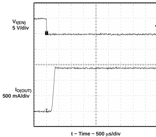
Figure 19. Short-Circuit Current, Device Enabled Into Short
