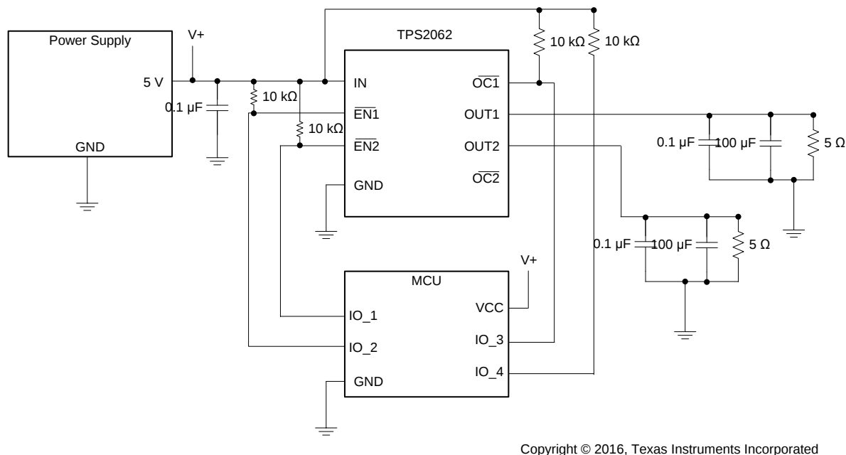
Figure 30. Typical Application Diagram
