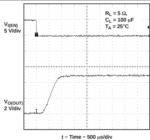
Figure 17. Turnon Delay and Rise Time With 100- \mu\text{F} Load
