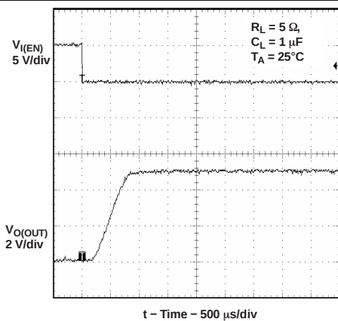
Figure 15. Turnon Delay and Rise Time With 1- \mu\text{F} Load
