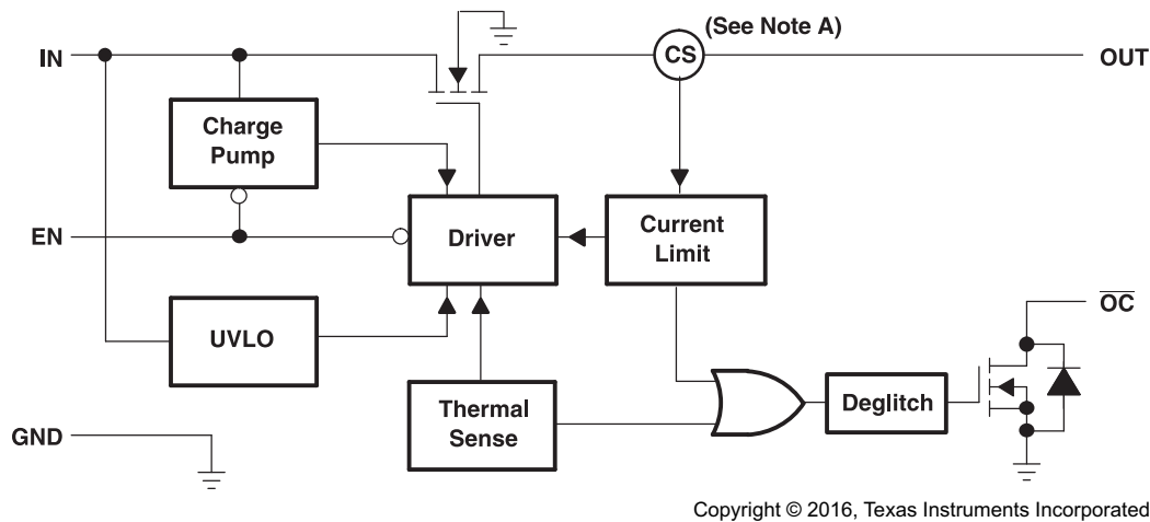
Figure 24. Functional Block Diagram – TPS2065-Q1
