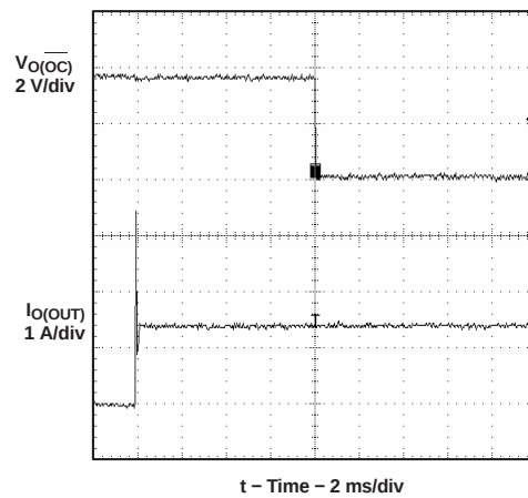
Figure 22. 1- \Omega Load Connected to Enabled Device
