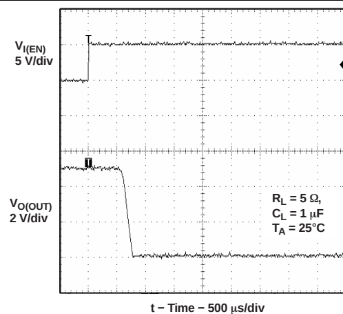
Figure 16. Turnoff Delay and Fall Time With 1- \mu\text{F} Load
