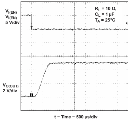
図 9-27. Turnon Delay and Rise Time With 1-μF Load
