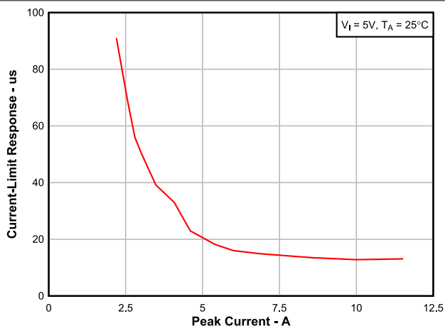
6-37. Current-Limit Response vs Peak Current
