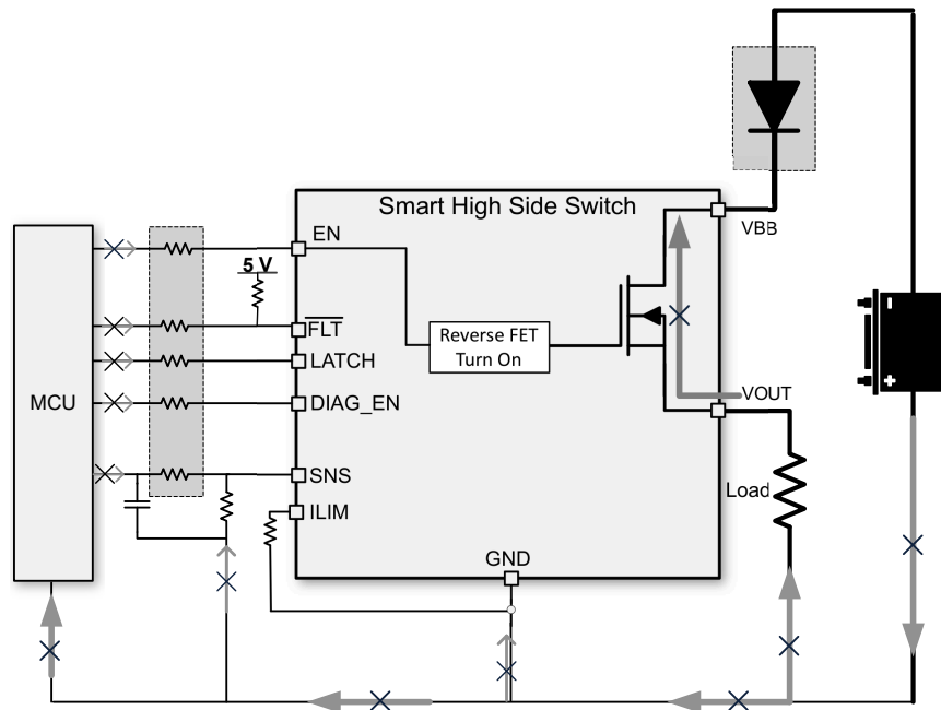
Figure 7-10. Reverse Protection With Blocking Diode
