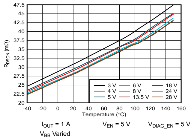
6-6. R_{DS(on)} vs Temperature
