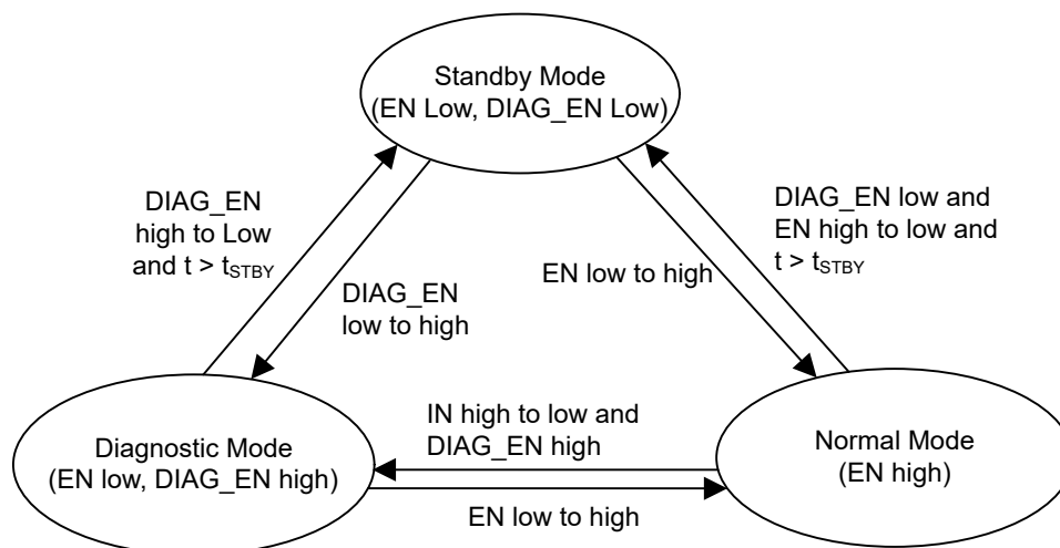
8-25. Work Mode State Machine
