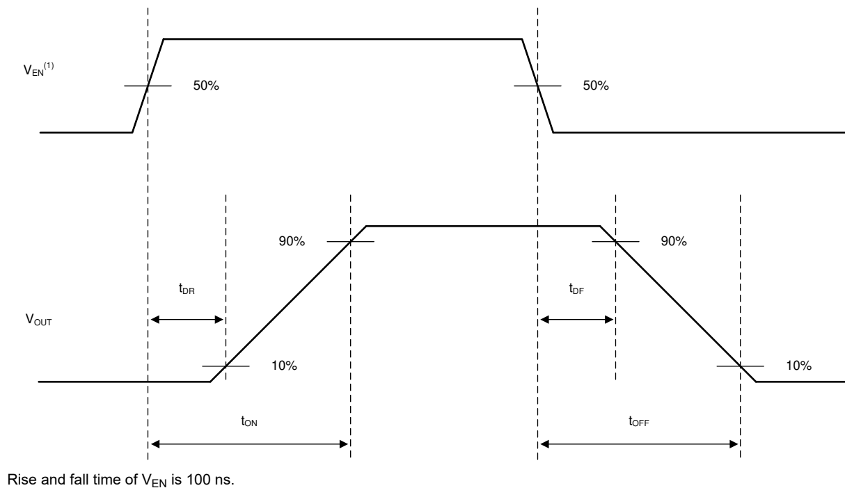
FIG 7-2. Switching Characteristics Definitions
