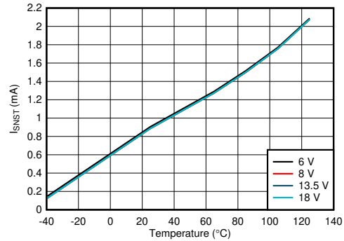
7-16. Temperature Sense Output Current ( I_{SNST} ) vs Temperature
