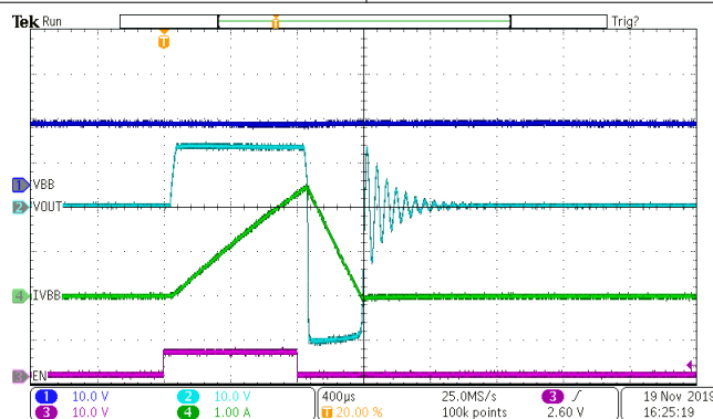
FIG 7-27. Device Version A Short Circuit Event
