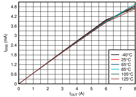
7-14. Current Sense Output Current ( I_{SNSI} ) vs Load Current ( I_{OUT} ) Across Temperature
