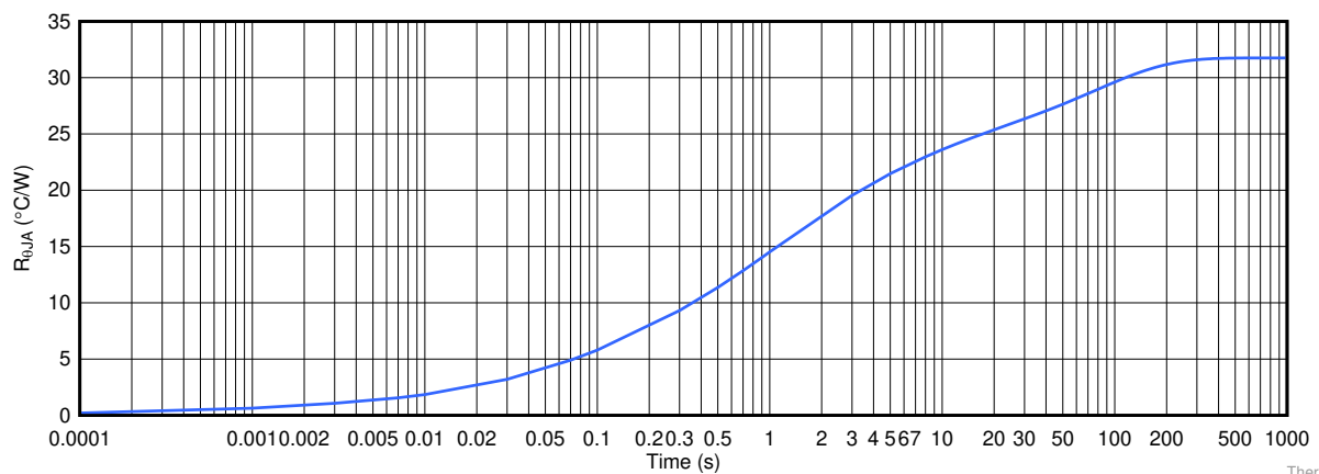
Figure 44. TPS1HB08-Q1 Transient Thermal Impedance
