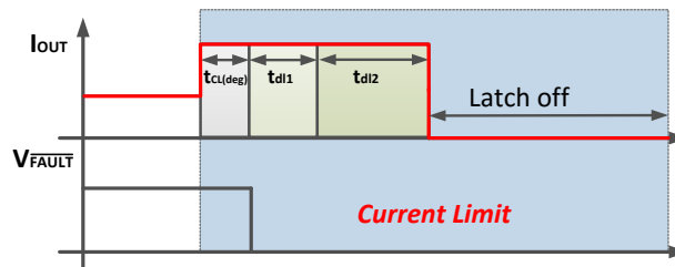
图 7-5. Latch-Off-Mode Example
