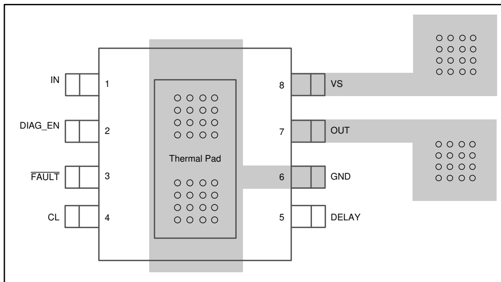
FIG 10-1. Layout Example
