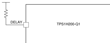
✎ 7-6. Auto-Retry-Mode Connection
