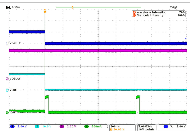
Figure 8-3. Hard-Short Condition in Auto-Retry Mode
