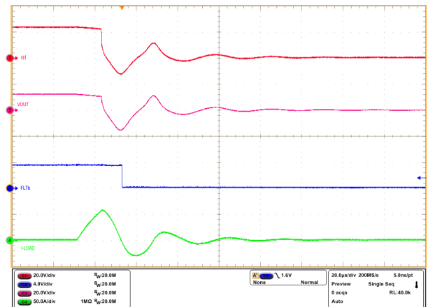
図 8-11. Output Short-Circuit Response of TPS1213-Q1
