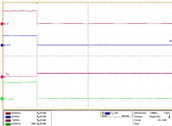
図 8-10. Latch-Off Response of TPS1213-Q1 for an Overcurrent Fault
