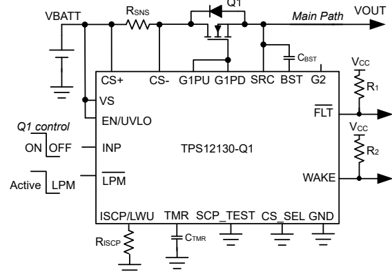
図 7-8. TPS12130-Q1 Application Circuit With External Sense Resistor R_{SNS} Based Current Sensing
