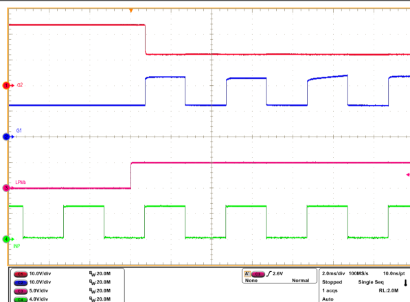
8-7. With \overline{\text{LPM}} = Low to High, INP Gained Control on G1 (VIN = 12V, No Load)
