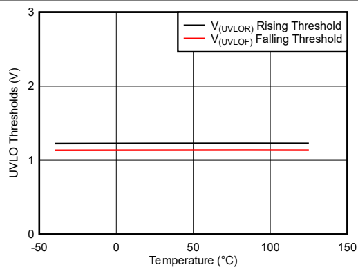
5-10. Input Supply UVLO Thresholds vs Temperature
