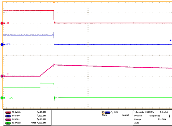
図 8-8. Overcurrent Response of TPS1213-Q1 EVM for 40A to 55A Load Step
