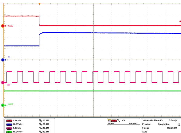
❏ 8-5. As \overline{\text{LPM}} = \text{Low} , INP Has No Control on G1 Even After WAKEUP
