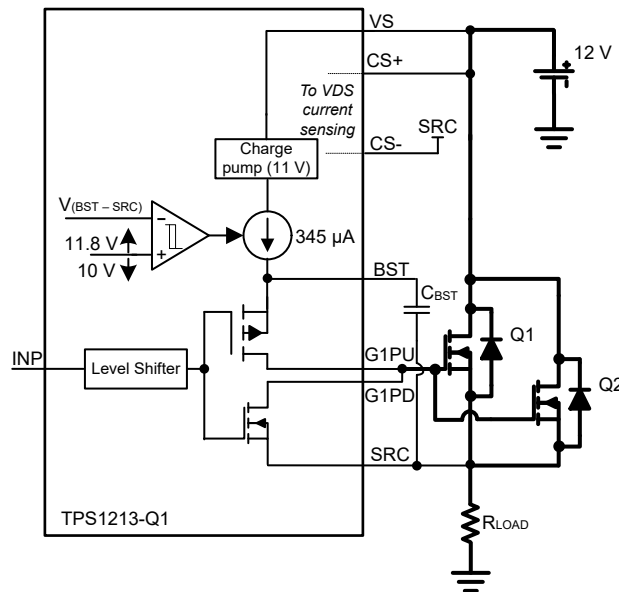
图 7-1. Main FET Gate Driver
