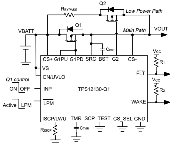
図 7-7. TPS12130-Q1 Application Circuit With Main FET RDSON Based Current Sensing
