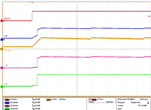
Figure 8-2. Start-Up Profile of Low Power Path (LPM = Low, VIN = 12V, No Load, CBST = 470nF)
