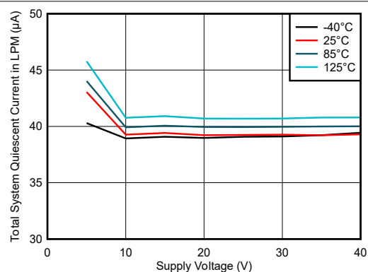
図 5-2. Operating Quiescent Current in LPM vs Supply Voltage
