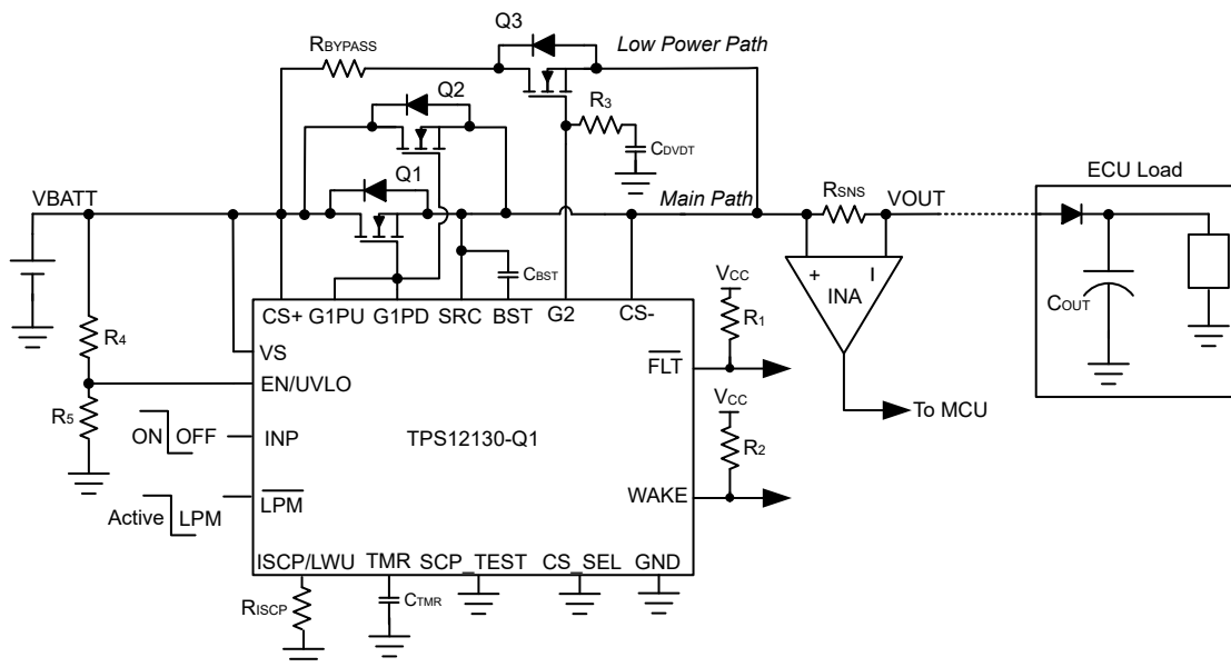
図 8-15. Always ON Automotive E-fuse With Bi-directional Current Sensing and Software I2t
