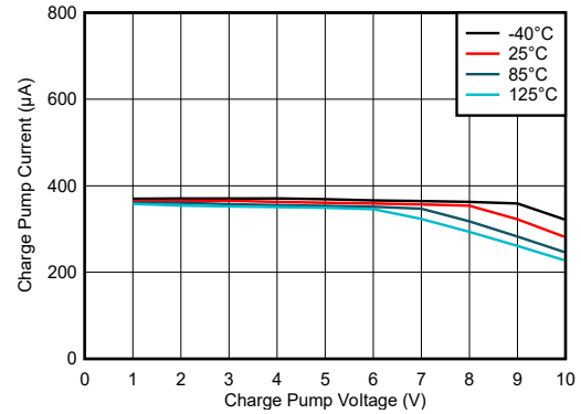
Figure 5-4. Charge Pump Current vs Charge Pump Voltage
