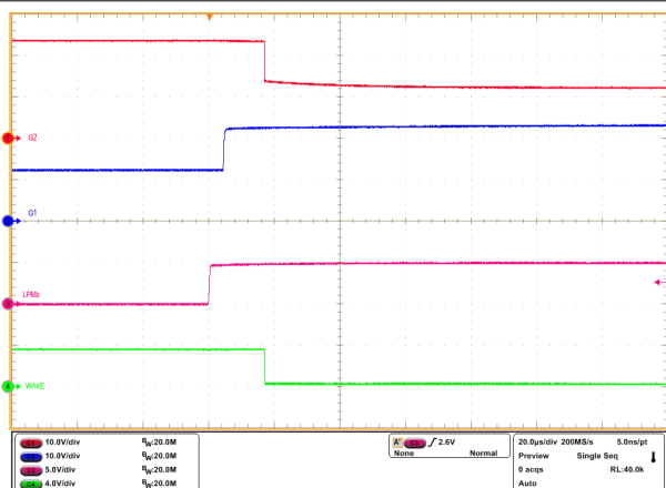
图 8-6. State Transition From LPM to Active Mode (LPM = Low to High, VIN = 12V, No Load)
