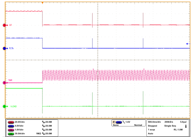
図 8-9. Auto-Retry Response of TPS1213-Q1 for an Overcurrent Fault
