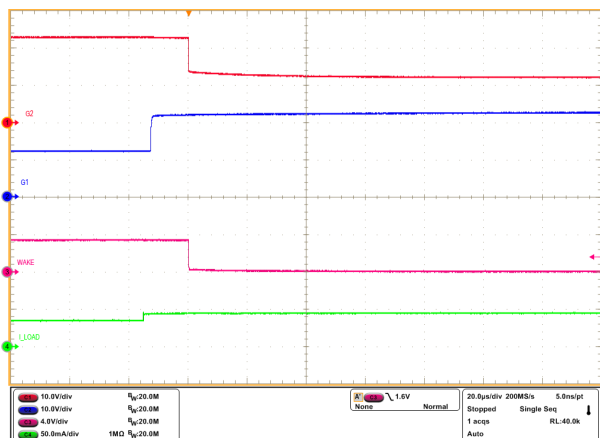
Figure 8-4. Zoom-In View of State Transition From LPM to Active Mode ( \overline{\text{LPM}} = Low, V_{\text{IN}} = 12\text{V} , \text{EN}/\text{UVLO} = High)
