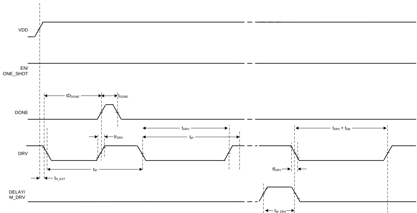
Figure 1. TPL5110 Timing
