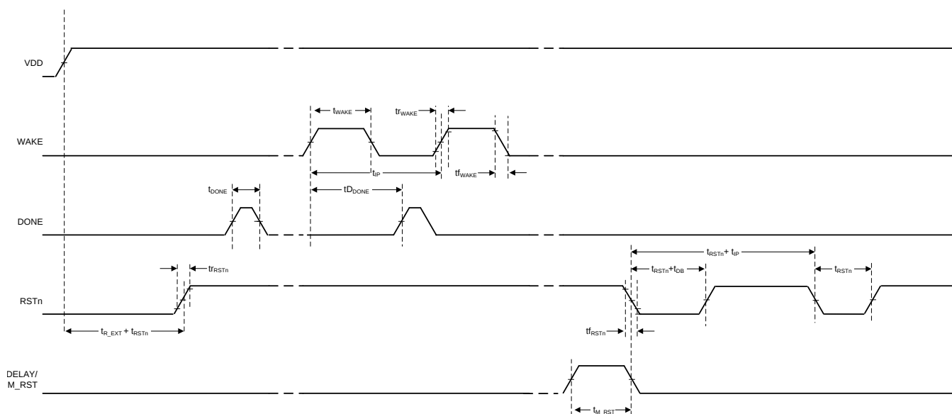
Figure 1. TPL5010 Timing
