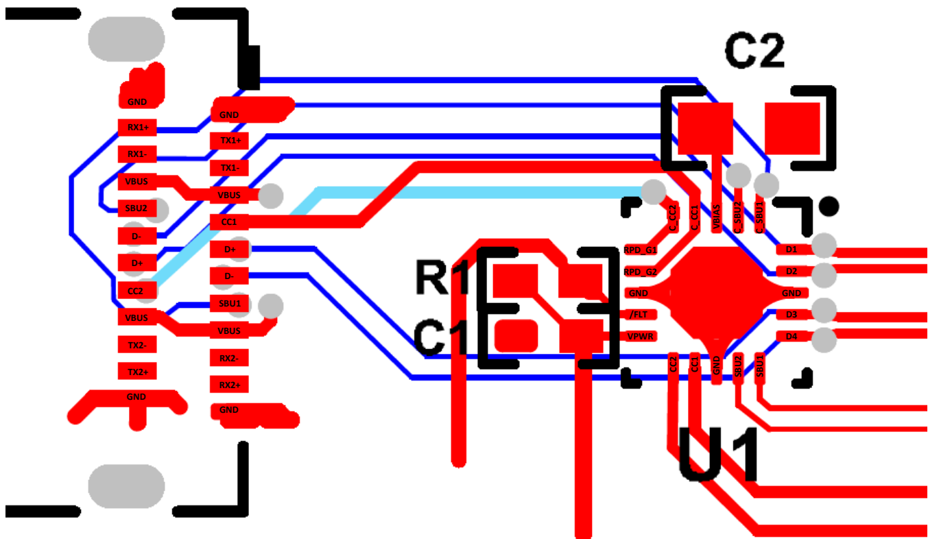
✎ 34. TPD8S300 Typical Layout
