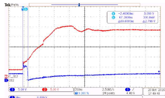
图 33. TPD6S300A Protecting the TPS65982 During a Short-to- V_{\text{BUS}} Event
