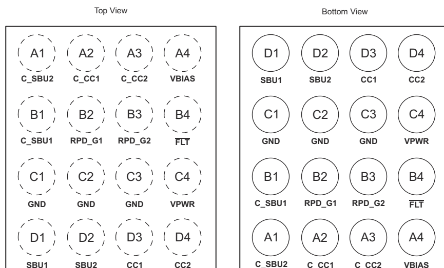
6-1. YBF Package 16-Pin DSBGA
