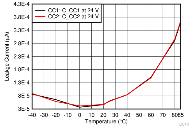
FIG 7-26. CC OVP Leakage Current vs Ambient Temperature at C_CC = 24 V
