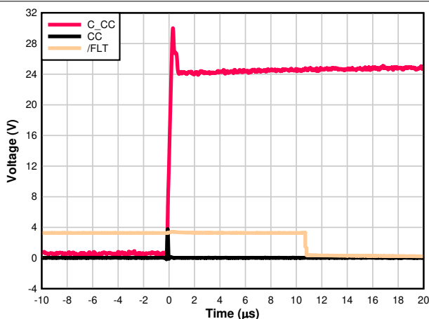
图 7-18. CC Short-to-V BUS 24 V Zoomed Out
