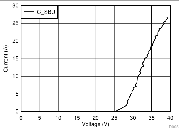
图 7-14. C_SBU TLP Curve Unpowered
