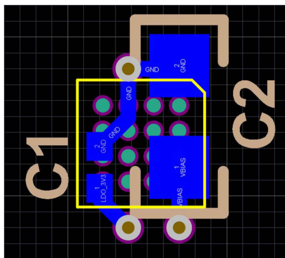
FIG 11-2. TPD4S311 Bottom Layer Routing
