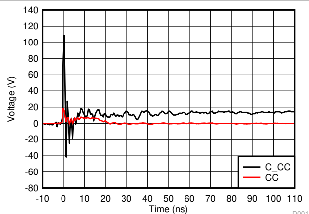
7-22. CC IEC 61000-4-2 8-kV Response Waveform
