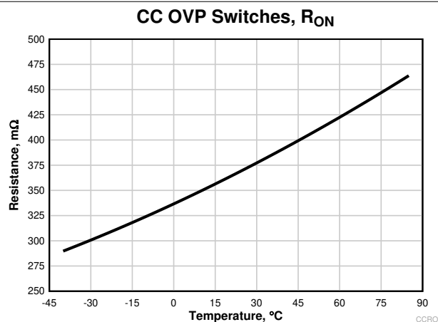
7-21. CC R_{ON} Versus Temperature
