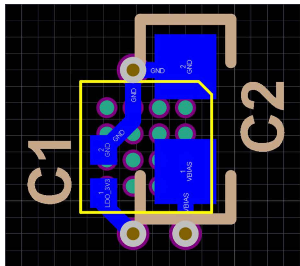
FIG 11-2. TPD4S311 Bottom Layer Routing
