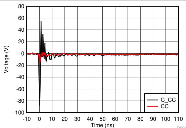
7-23. CC IEC 61000-4-2 -8-kV Response Waveform
