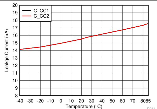
7-24. C_{CC} Path Leakage Current vs Ambient Temperature at C_{CC} = 5.5 V
