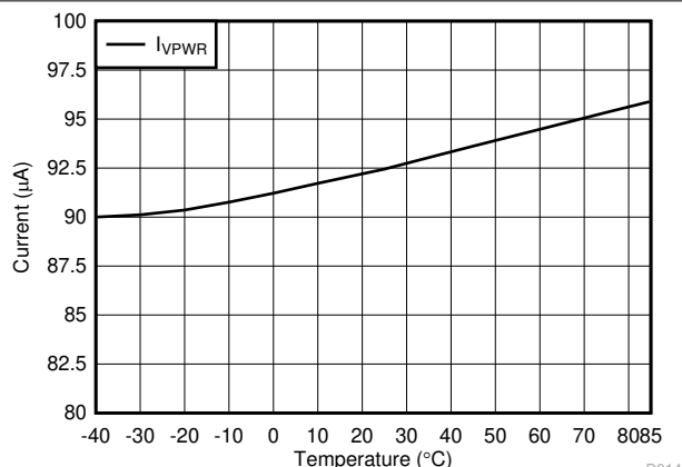
FIG 7-30. V_PWR Supply Leakage vs Ambient Temperature at 3.6 V
