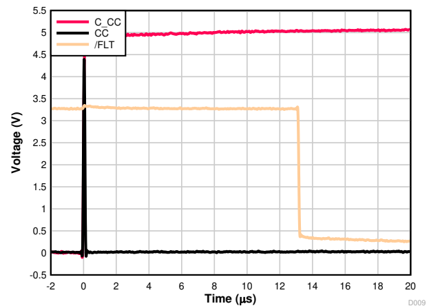
7-20. CC Short-to- V_{BUS} 5 V Zoomed Out
