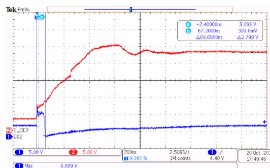
9-4. TPD4S311 Protecting the TPS65982 During a Short-to- V_{BUS} Event
