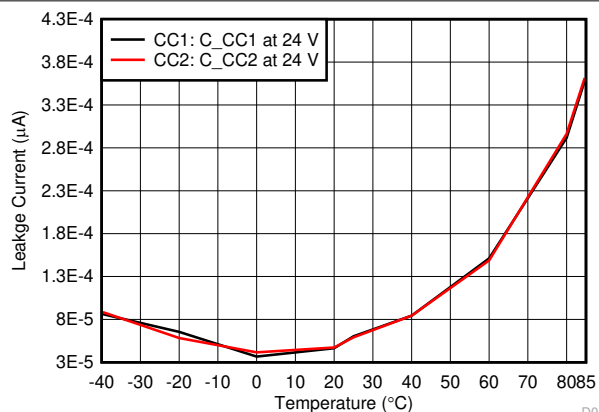
FIG 7-26. CC OVP Leakage Current vs Ambient Temperature at C_CC = 24 V
