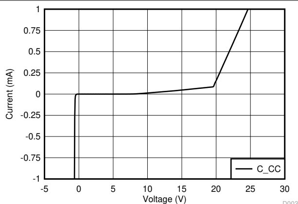
FIG 7-29. C_CC IV Curve
