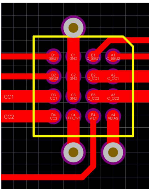
FIG 11-1. TPD4S311 Top Layer Routing
