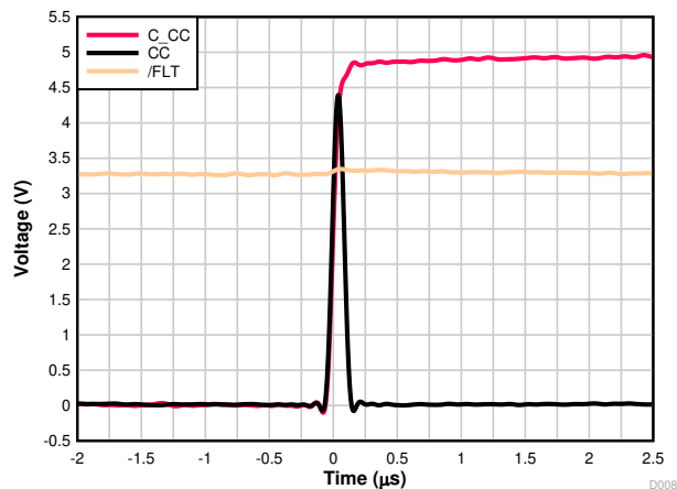
7-19. CC Short-to- V_{BUS} 5 V Zoomed In
