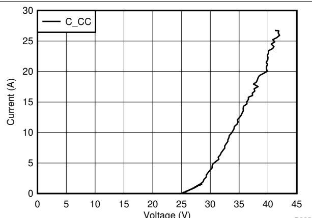
FIG 7-28. C_CC TLP Curve Unpowered
