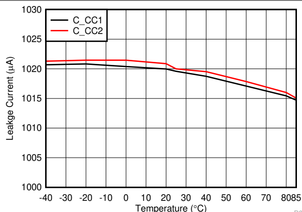
FIG 7-25. C_CC OVP Leakage Current vs Ambient Temperature at C_CC = 24 V
