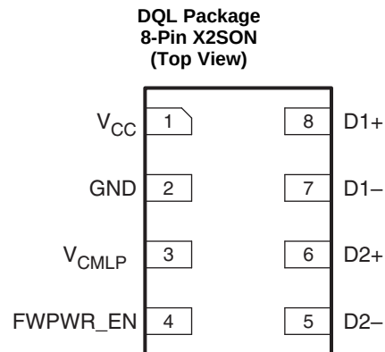
Pin Functions
