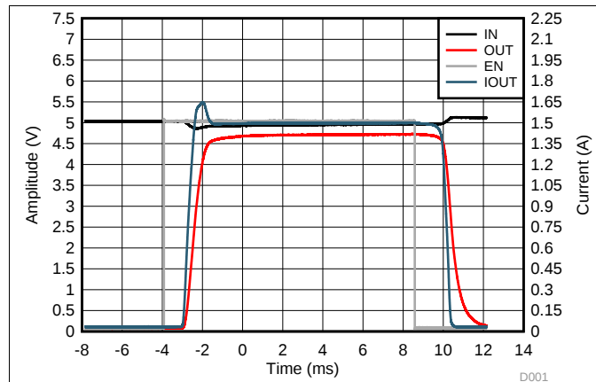
Figure 6. TPD3S044 Turn-On into 3.3 \Omega
