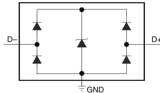
7-2. TPD2EUSB30/A Circuit
