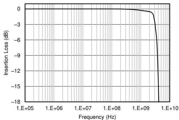
FIG 6-9. Insertion Loss
