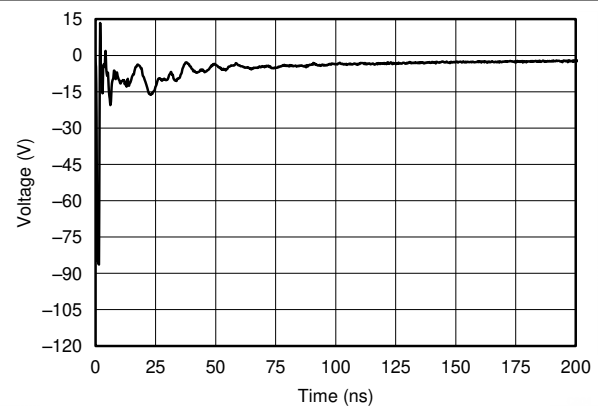
FIG 6-4. IEC 61000-4-2 Clamping Voltage, -8-kV Contact
