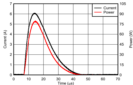
FIG 6-8. Surge Curve ( t_p = 8/20\text{ }\mu\text{s} ) IO to GND
