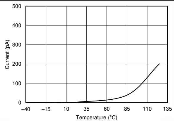
FIG 6-6. I_{\text{LEAK}} vs Temperature, V_{\text{IN}} = 2.5\text{ V}
