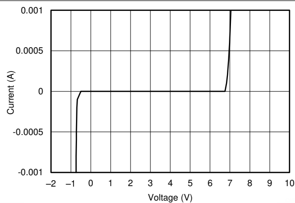
FIG 6-5. IV Curve, T_A = 25^\circ\text{C}
