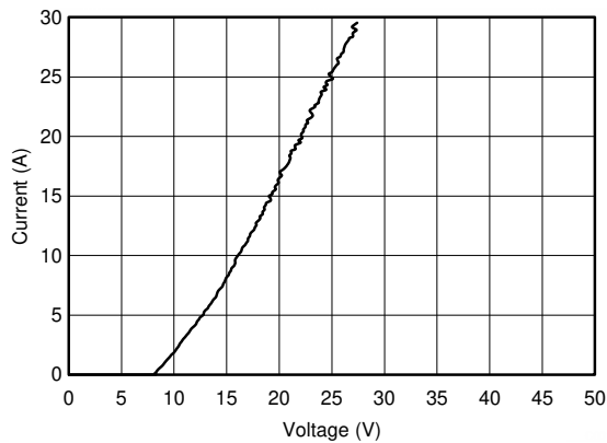
FIG 6-1. TLP, Data to GND
