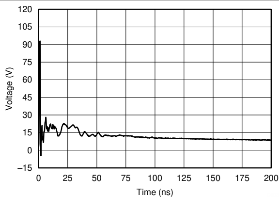
FIG 6-3. IEC 61000-4-2 Clamping Voltage, 8-kV Contact
