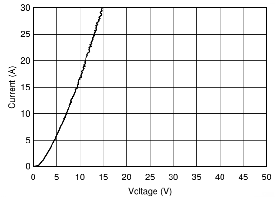
FIG 6-2. TLP, GND to Data
