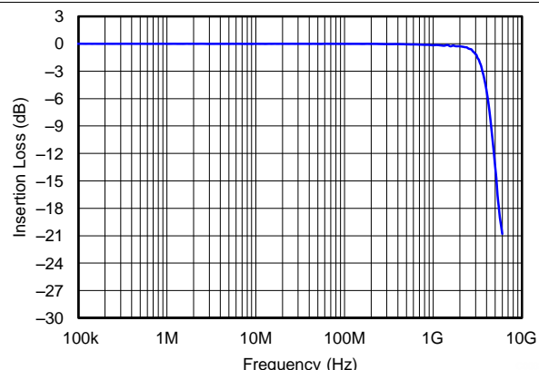
Figure 6. Insertion Loss
