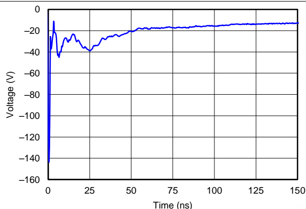
Figure 5. -8-kV Contact ESD Clamping
