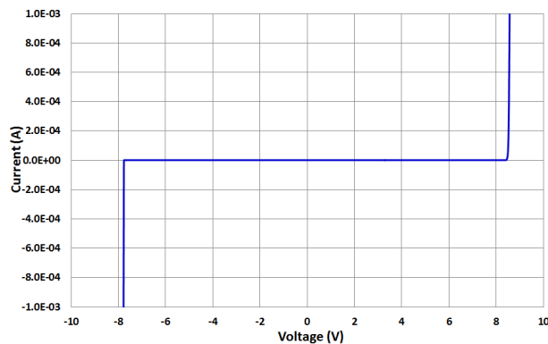
FIG 6-5. IV Curve
