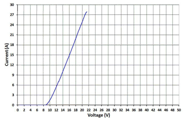
FIG 6-4. Transmission Line Pulse (TLP) Waveform Pin 2 to Pin 1
