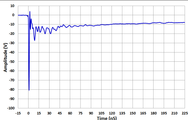
8-3. IEC 61000-4-2 Clamp Voltage -8-kV Contact ESD
