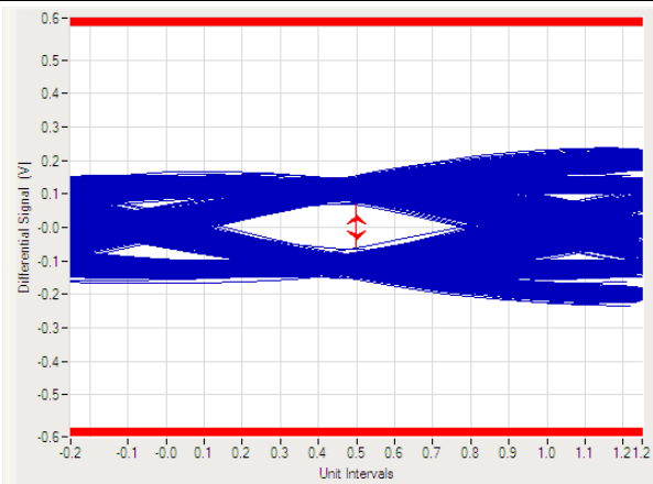
Figure 12. USB3.1 Gen 2 10-Gbps Eye Diagram (Bare Board)
