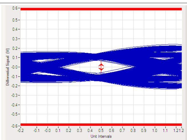
Figure 16. USB 3.1 Gen 2 10-Gbps Eye Diagram (with TPD1E0B04DPL)
