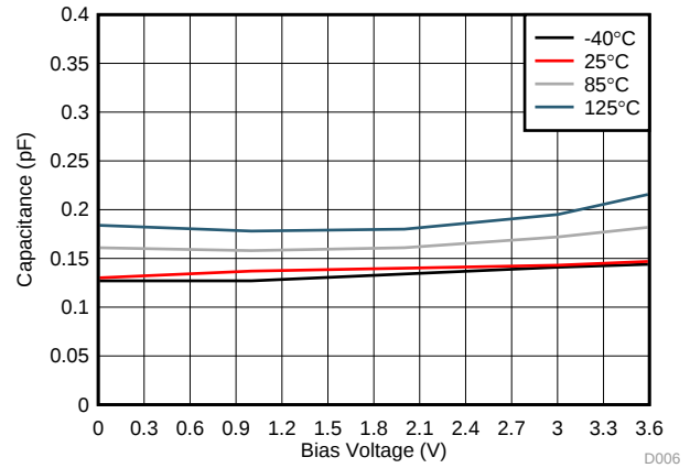
Figure 20. Capacitance vs. Bias Voltage
