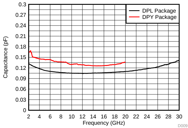
Figure 19. Capacitance vs. Frequency
