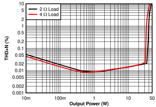
Figure 6-38. THD+N vs Power - 2 \Omega , 4 \Omega - 18 V
