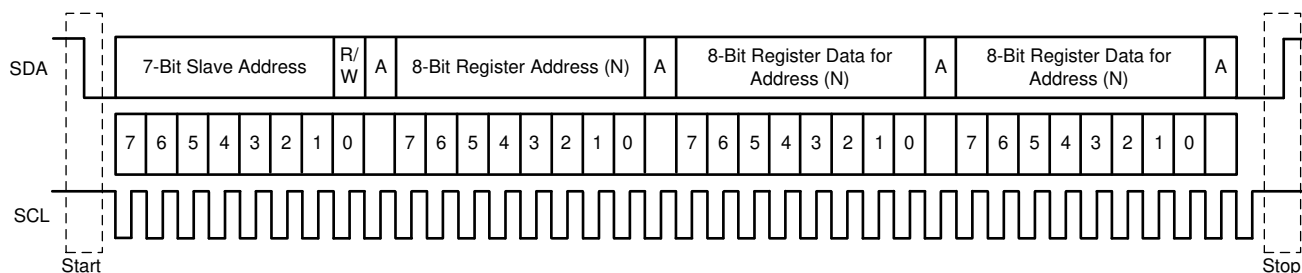
FIG 7-8. Typical I 2 C Sequence
