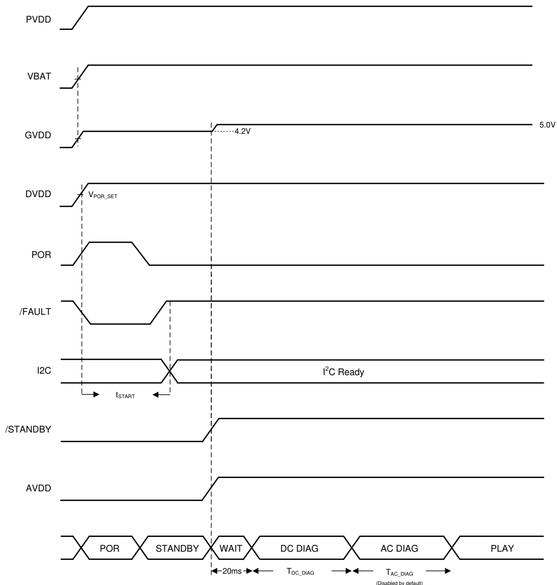
☒ 7-4. Typical Initialization Sequence and Timing
