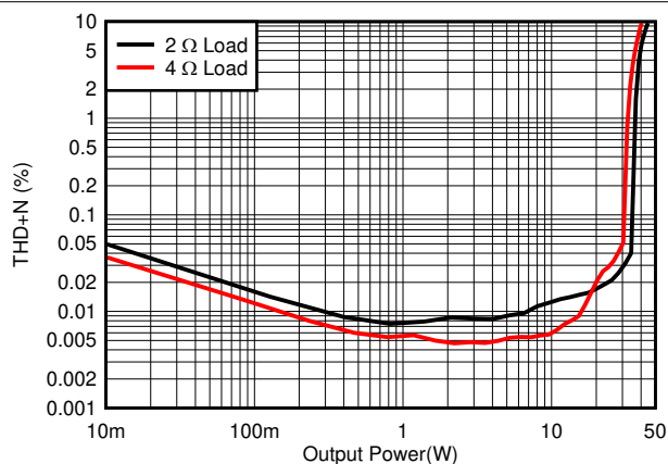
FIG 6-2. THD+N vs Power - 2 \Omega , 4 \Omega - 18 V
