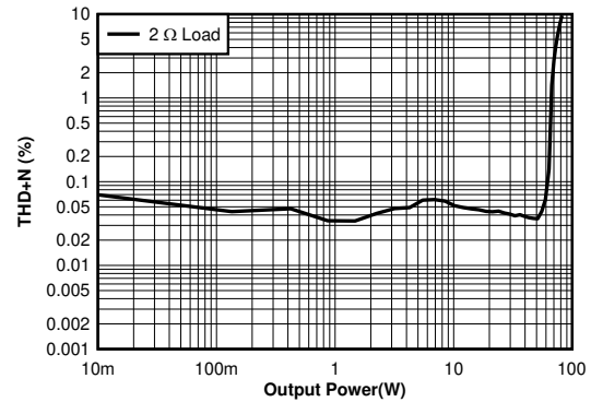
Figure 6-19. THD+N vs Power - PBTL, 2 Ω, 18 V
