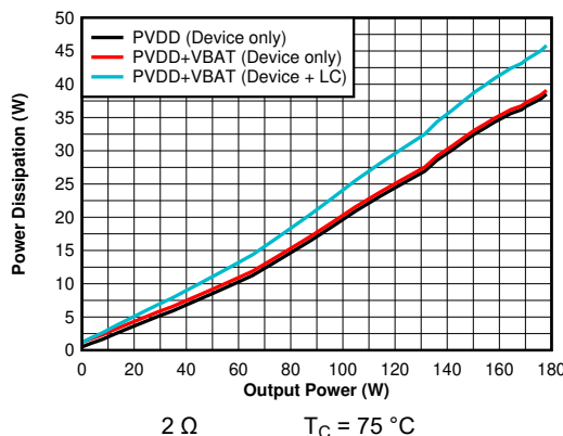
Figure 6-58. Power Dissipation vs Output Power - 2 \Omega
