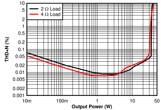
FIG 6-26. THD+N vs Power - BTL, 2 \Omega , 4 \Omega , 18 V, 1SPW
