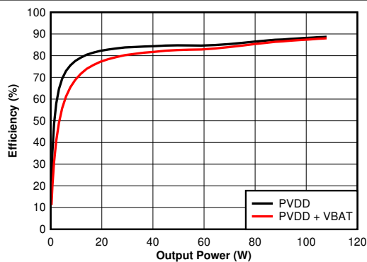
FIG 6-5. Efficiency vs Output Power - 4 \Omega
