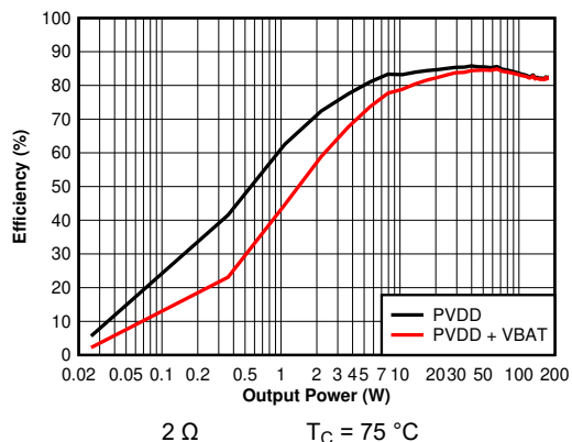
Figure 6-57. Efficiency vs Output Power - 2 \Omega (Zoomed)
