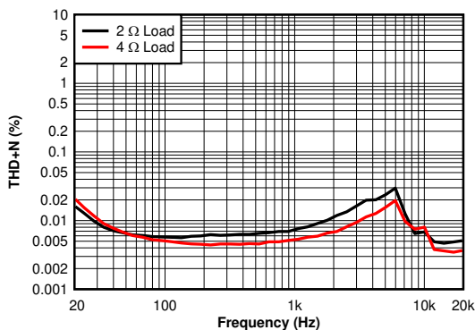
FIG 6-3. THD+N vs Frequency - 2 \Omega , 4 \Omega
