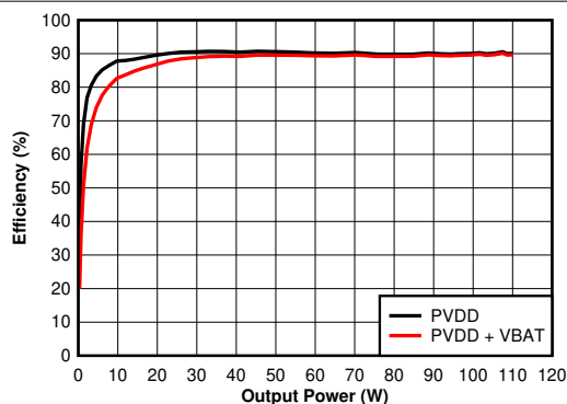
Figure 6-53. Efficiency vs Output Power - 4 \Omega
