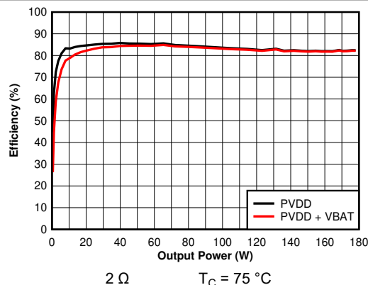
Figure 6-56. Efficiency vs Output Power - 2 \Omega
