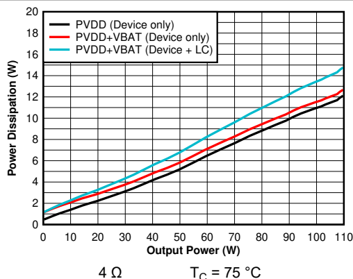
Figure 6-55. Power Dissipation vs Output Power - 4 \Omega
