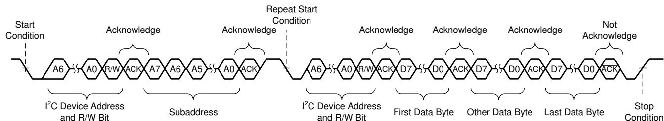
FIG 7-13. Sequential Read Transfer
