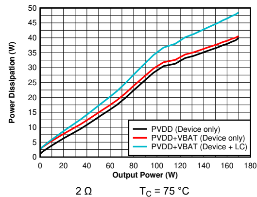
Figure 6-10. Power Dissipation vs Output Power - 2 \Omega
