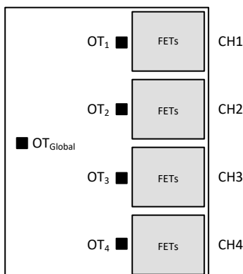
FIG 7-5. Temperature Sensor Locations Within the Device
