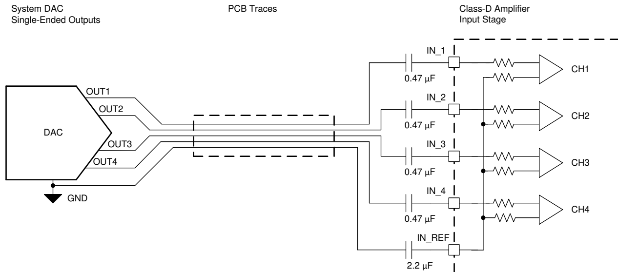
FIG 7-1. Single-Ended Analog Input Connections
