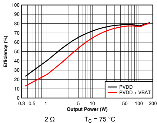
Figure 6-9. Efficiency vs Output Power - 2 \Omega (Zoomed)
