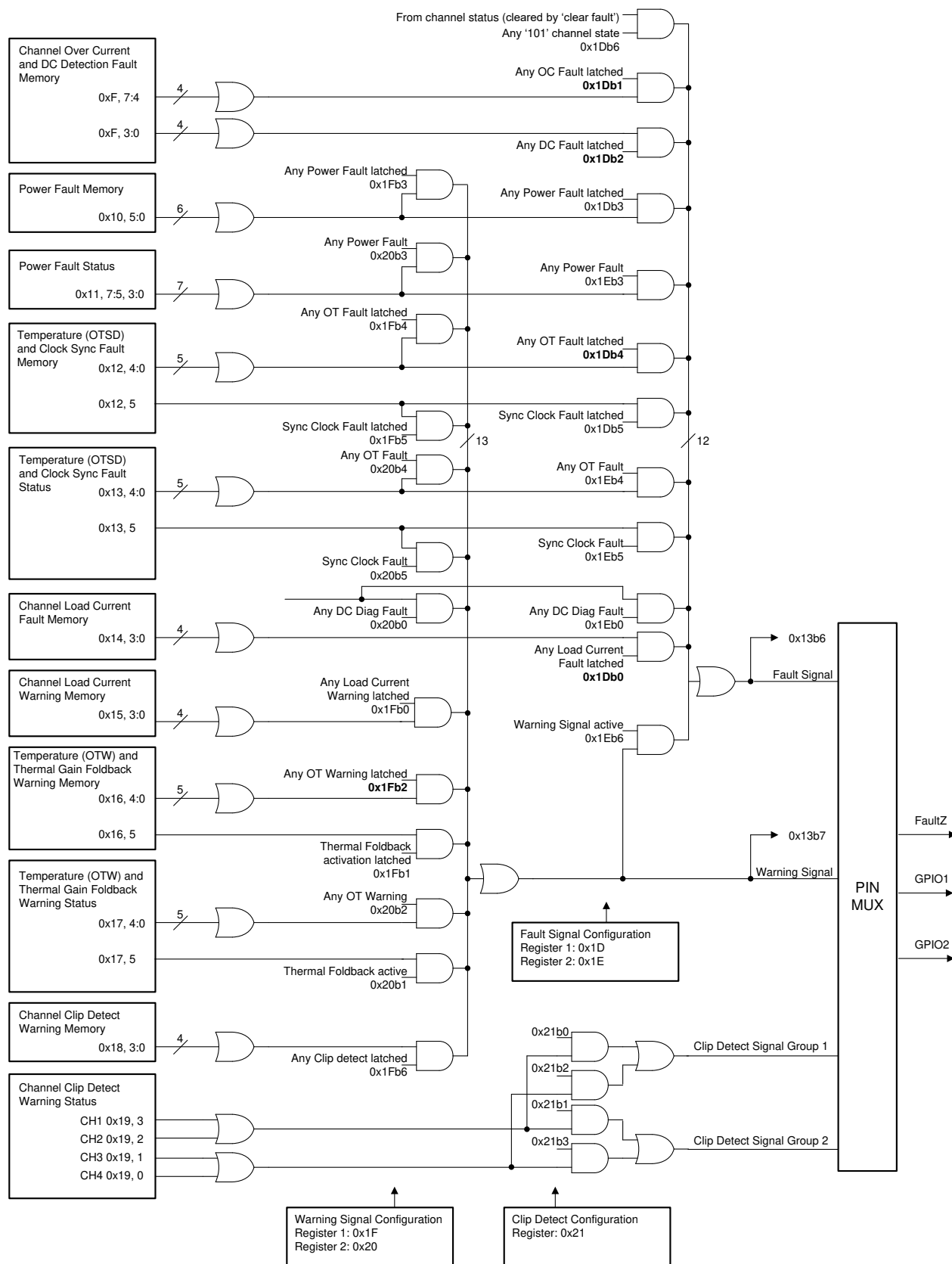
7-7. Fault, Warning and Clip Detect Signal Creation and Configuration
