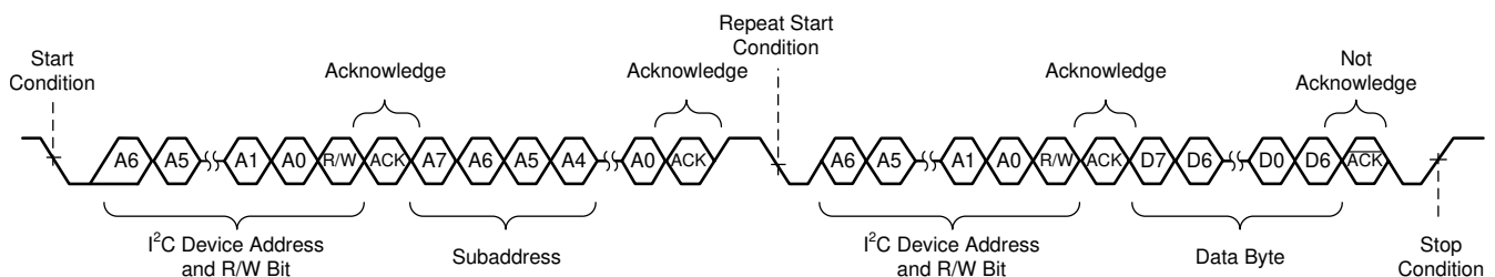
FIG 7-12. Random Read Transfer
