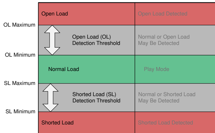
FIG 7-3. DC Load Diagnostic Reporting Thresholds
