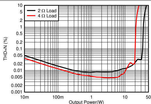
FIG 6-1. THD+N vs Power - 2 \Omega , 4 \Omega - 14.4 V
