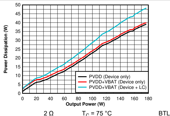
Figure 6-32. Power Dissipation vs Output Power - BTL, 2 \Omega , 14.4 V, 1SPW
