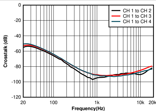
6-14. Crosstalk vs Frequency
