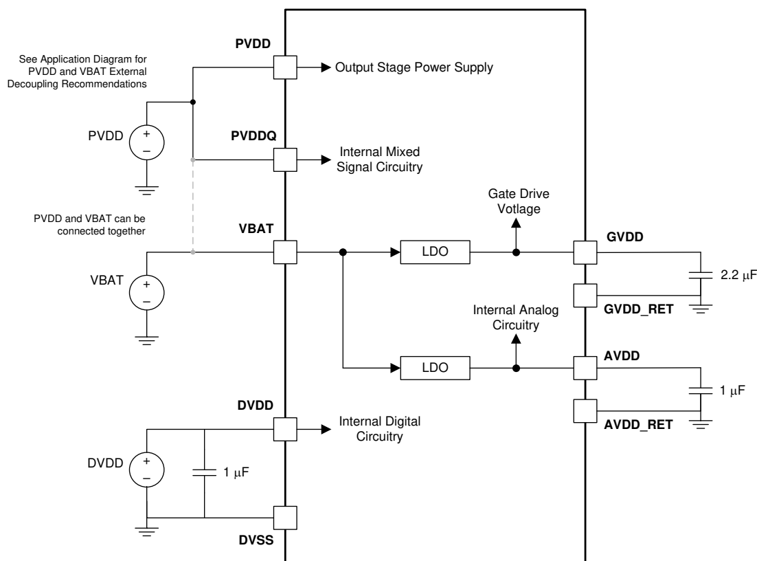
9-1. Power Supply Block
